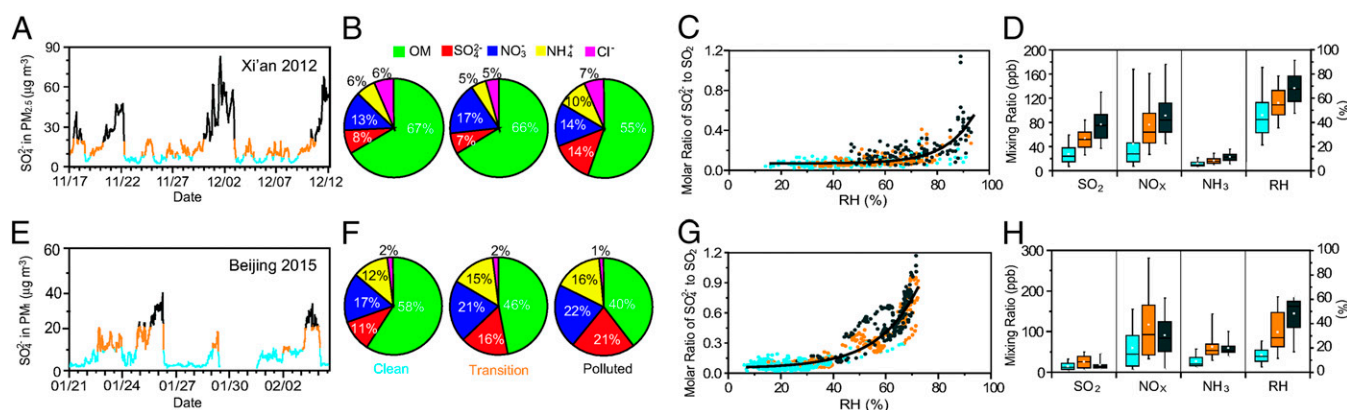
Fig. 1. Sulfate production during pollution episodes in Xi'an and Beijing. (A–D) Measurements in Xi'an from 17 November to 12 December 2012, and the particle properties correspond to those in PM 2.5 . (E–H) Measurements in Beijing from 21 January to February 4, 2015, and the particle properties correspond to those in PM 1 (particles smaller than 1 μm). In A and E, the dates on the x axis correspond to midnight local time. B and F show the mass fractions of the five main nonrefractory constituents from 5 to 12 December 2012 in Xi'an and from 21 January to 4 February 2015 in Beijing, respectively. The lines in C and G represent the exponential fits through the data, i.e., y = 0.07 + 1.0 \times 10^{-4} \exp(x/11) with R^2 = 0.60 in Xi'an and y = 0.05 + 7.0 \times 10^{-3} \exp(x/15) with R^2 = 0.88 in Beijing. Except for the colors in B and F depicting the aerosol compositions, the blue, orange, and black colors correspond to the SO 4 2- mass concentrations of less than 10 μg m -3 (clean), 10–20 μg m -3 (transition), and greater than 20 μg m -3 (polluted), respectively. The top and bottom of the vertical line for each box in D and H correspond to the 95th and 5th percentiles, respectively, and the top, middle, and bottom horizontal lines of the box mark the 75th, 50th, and 25th percentiles of the data range. The white dot in each box represents the mean value.
