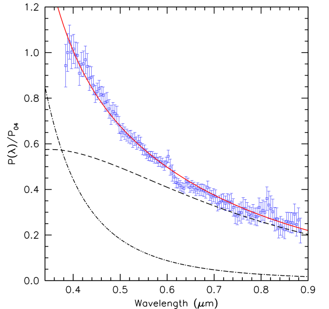
Fig. 6. Illustrative decomposition of the observed polarization in SN 2014J using a Serkowski law (dashed) and a Rayleigh law (dotted-dashed). The solid line fitting the data traces the sum of the two (see text).
