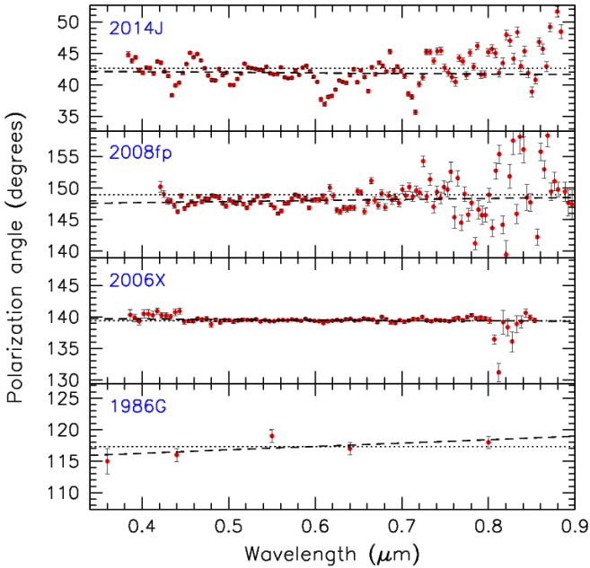
Fig. 1. Polarization angles for the SNe in the sample. The dashed lines trace the weighted linear best fit ( \lambda \leq 0.8 \mu\text{m} ), while the dotted lines indicate the average value computed using the full wavelength range.
