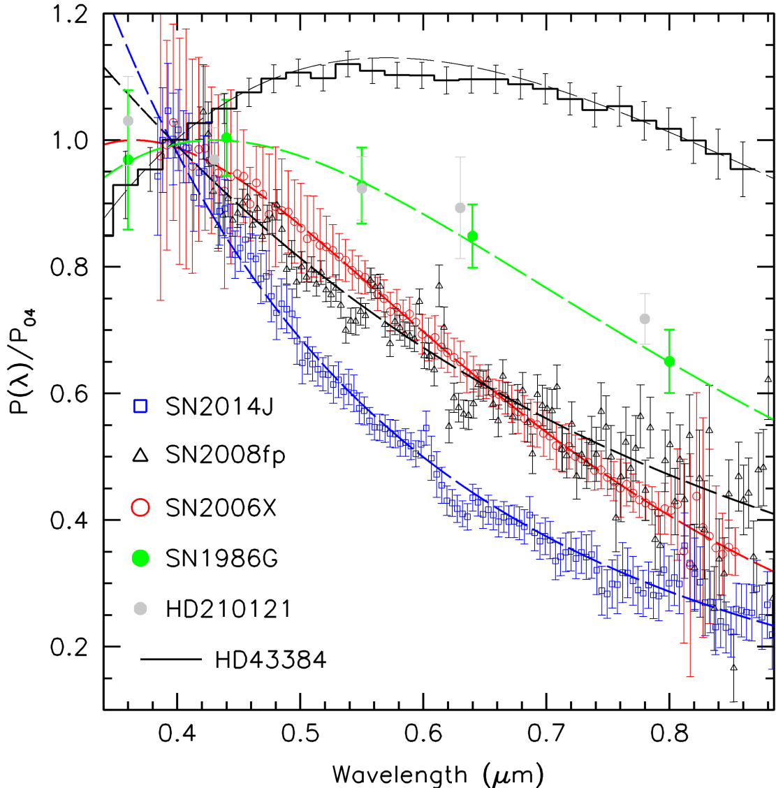
Fig. 2. Observed polarization wavelength dependence for SN 1986G (Hough et al. 1987), SN 2006X (Patat et al. 2009), SN 2008fp (Cox & Patat 2014a), and SN 2014J (this work). For comparison, the data of HD 43384 (this work) and HD 210121 (Larson et al. 1996) are also plotted. The dashed curves trace Serkowski law best fits. For presentation, the curves were normalized to P_{04} (see text). The error bars were kept at their original values. HD 43384 is a polarized standard; HD 210121 is a Galactic star with very low R_V . For SNe 2006X, 2008fp and 2014J, P(\lambda) was computed as the polarization component parallel to the polarization angle.
