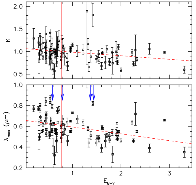
Fig. 4. Serkowski parameters K and \lambda_{max} as a function of E_{B-V} for the Whittet et al. (1992) sample. The dashed lines trace the best linear least-squares fit to the data. The vertical solid line marks the median E_{B-V} , while the arrows are placed at the values of the four SN (see Table 1).
