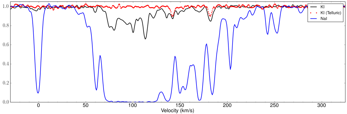
Fig. 5. Galactic and interstellar absorption components for Na I D (blue) and K I (black). The dotted curve traces a telluric absorption spectrum for the K I region. The data were obtained with the HERMES spectrograph (Sternberg et al. 2014.)
