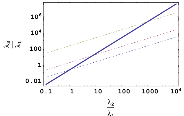
FIG. 1. The solid line corresponds to the condition in Eq. (4). The dashed lines represent \lambda_1 = \text{const.} contours corresponding to density perturbations condition (6) for \lambda_1 = 1 \times 10^{-8} , 5 \times 10^{-9} , 1 \times 10^{-9} respectively (from bottom to top).
