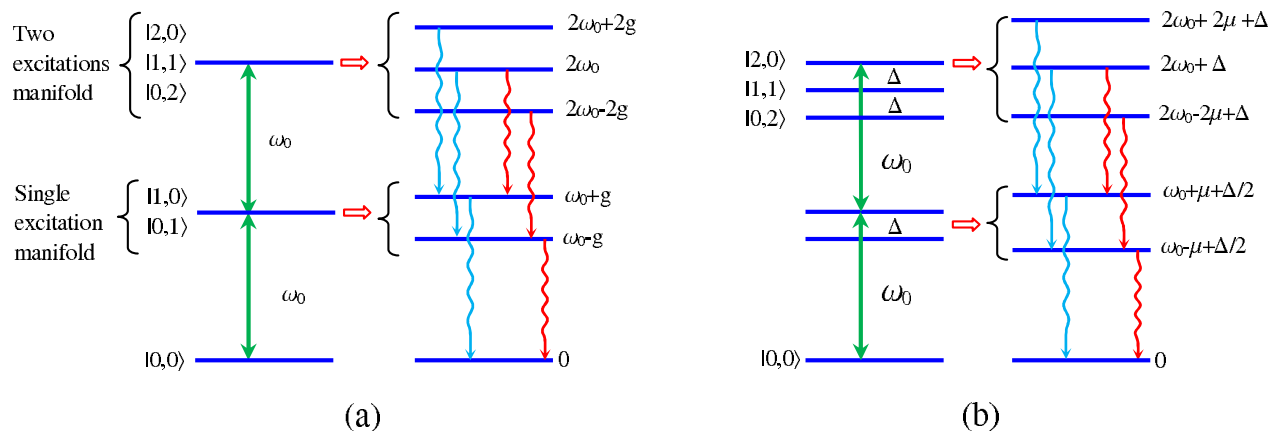
FIG. 7: (a) Dressed state energy level diagram for single and two excitation manifolds when the exciton is at resonance with photon. (b) Dressed states energy level diagram when the exciton frequency is detuned by \Delta from that of the photon. We have assumed \Delta to be positive for sake of simplicity. The bare states |n, m\rangle ( n, m = 0, 1, 2 ) represent n numbers of excitons and m numbers of photons. Even though there are 6 possible transitions there are only 2 distinct transition frequencies namely: \omega - \omega_0 = \mu + \Delta/2 and \omega - \omega_0 = -\mu + \Delta/2 , where \mu = \sqrt{g^2 + \Delta^2/4} .
