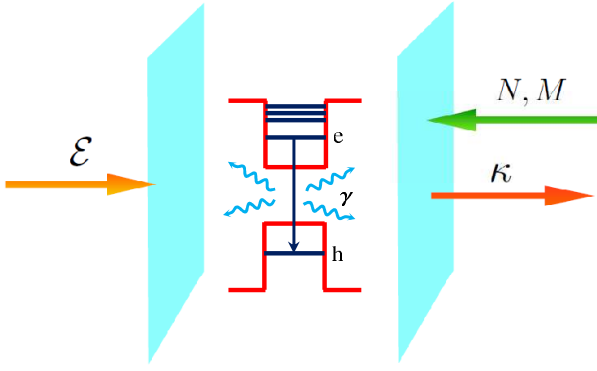
FIG. 1: Schematic representation of a quantum well (QW) in a driven cavity coupled to a squeezed vacuum reservoir.
