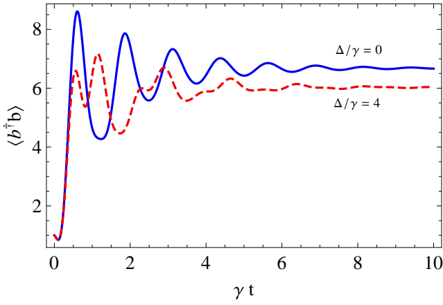
FIG. 4: Plots of the fluorescent intensity [Eq. (20)] vs scaled time \gamma t for \kappa/\gamma = 1.2, g/\gamma = 5, r = 1.8, \text{pump amplitude } \varepsilon/\gamma = 7 and for different values of exciton-photon detuning ( \Delta/\gamma ).
