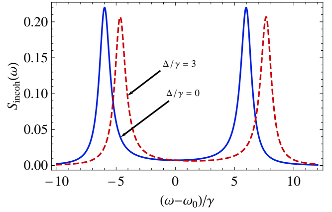
FIG. 5: Plots of the incoherent component of the power spectrum [Eq. (26)] vs scaled frequency (\omega - \omega_0)/\gamma for \kappa/\gamma = 1.2, g/\gamma = 6, \text{ and squeeze parameter } r = 1 , and for different values of detuning, \Delta/\gamma .
