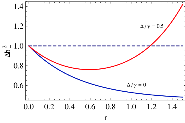
FIG. 9: Plots of the steady state quadrature variance [(35)] vs squeeze parameter r for g/\gamma = 5 , \kappa/\gamma = 1.2 , and for the different values of exciton-photon detuning \Delta/\gamma .
