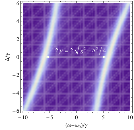
FIG. 6: Density plot of the incoherent component of the power spectrum [Eq. (26)] vs scaled frequency (\omega - \omega_0)/\gamma and \Delta/\gamma for \kappa/\gamma = 1.2, g/\gamma = 6, \text{ and squeeze parameter } r = 1 .
