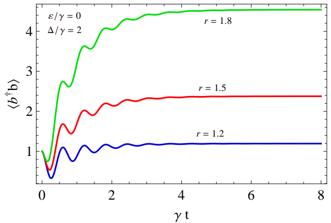
FIG. 3: Plots of the fluorescent intensity [Eq. (22)] vs scaled time \gamma t for \kappa/\gamma = 1.2, g/\gamma = 5, \Delta/\gamma = 2 , not external driving field ( \varepsilon/\gamma = 0 ) and for different values of r .
