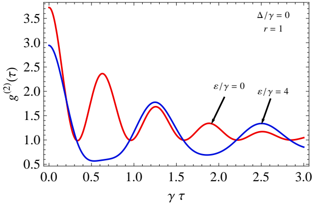
FIG. 8: Plot of second-order correlation function versus normalized time \gamma\tau for g/\gamma = 5 , \kappa/\gamma = 1.2 , \Delta/\gamma = 0 , squeezing parameter r = 1 , and for different value of pump amplitude \varepsilon/\gamma .
