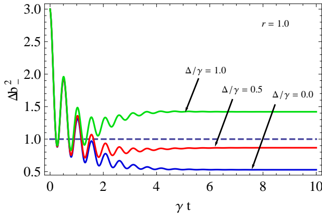
FIG. 10: Plots of the quadrature variance [(33)] vs scaled time \gamma t for g/\gamma = 5 , \kappa/\gamma = 1.2 , squeeze parameter r = 1 and for the different values of exciton-photon detuning \Delta/\gamma .
