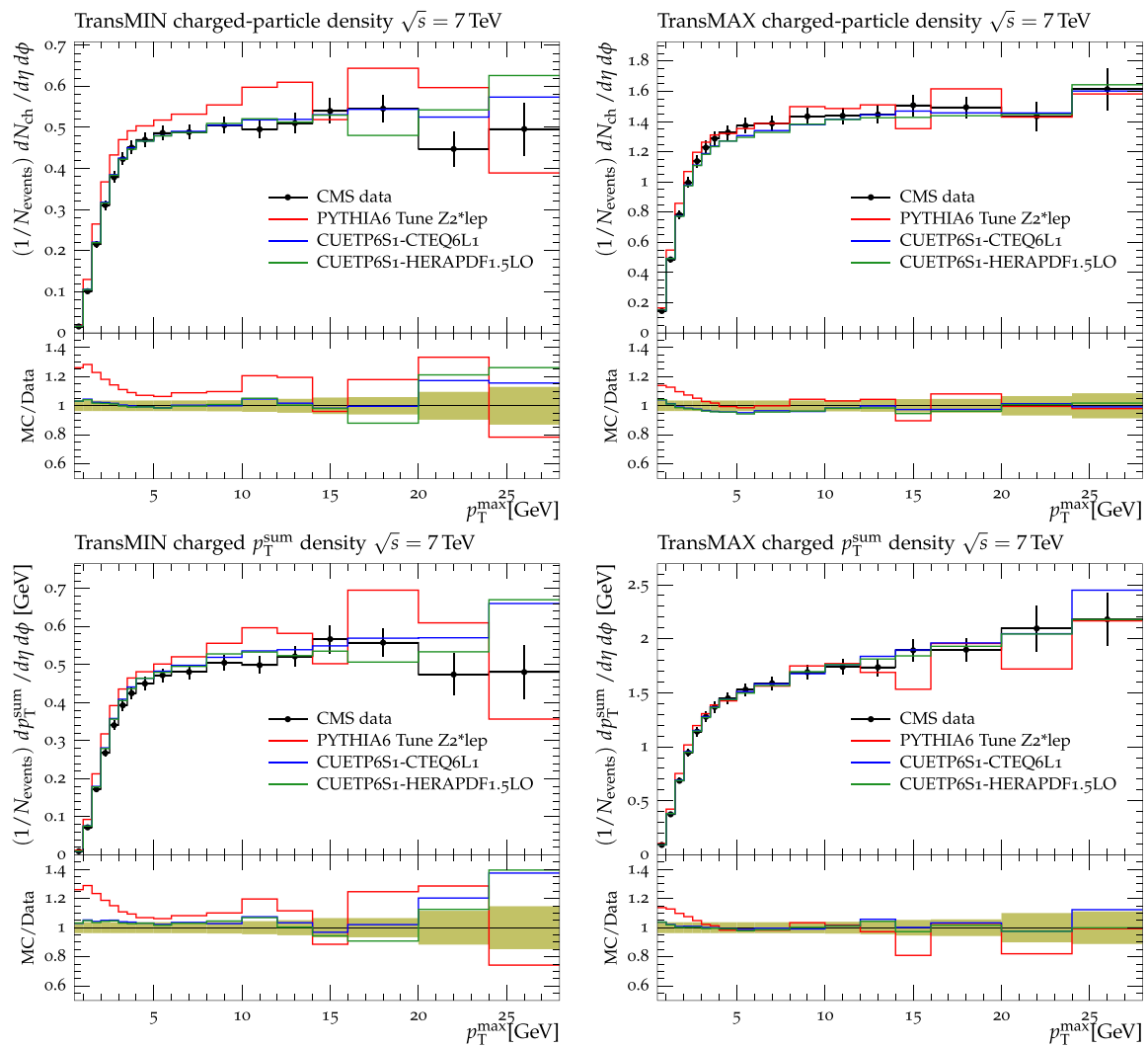
Fig. 26 CMS data at \sqrt{s} = 7 \text{ TeV} [17] on the particle ( top ) and p_T^{\text{sum}} densities ( bottom ) for charged particles with p_T > 0.5 \text{ GeV} and |\eta| < 0.8 in the TransMIN ( left ) and TransMAX ( right ) regions as defined by the leading charged particle, as a function of the transverse momen-
