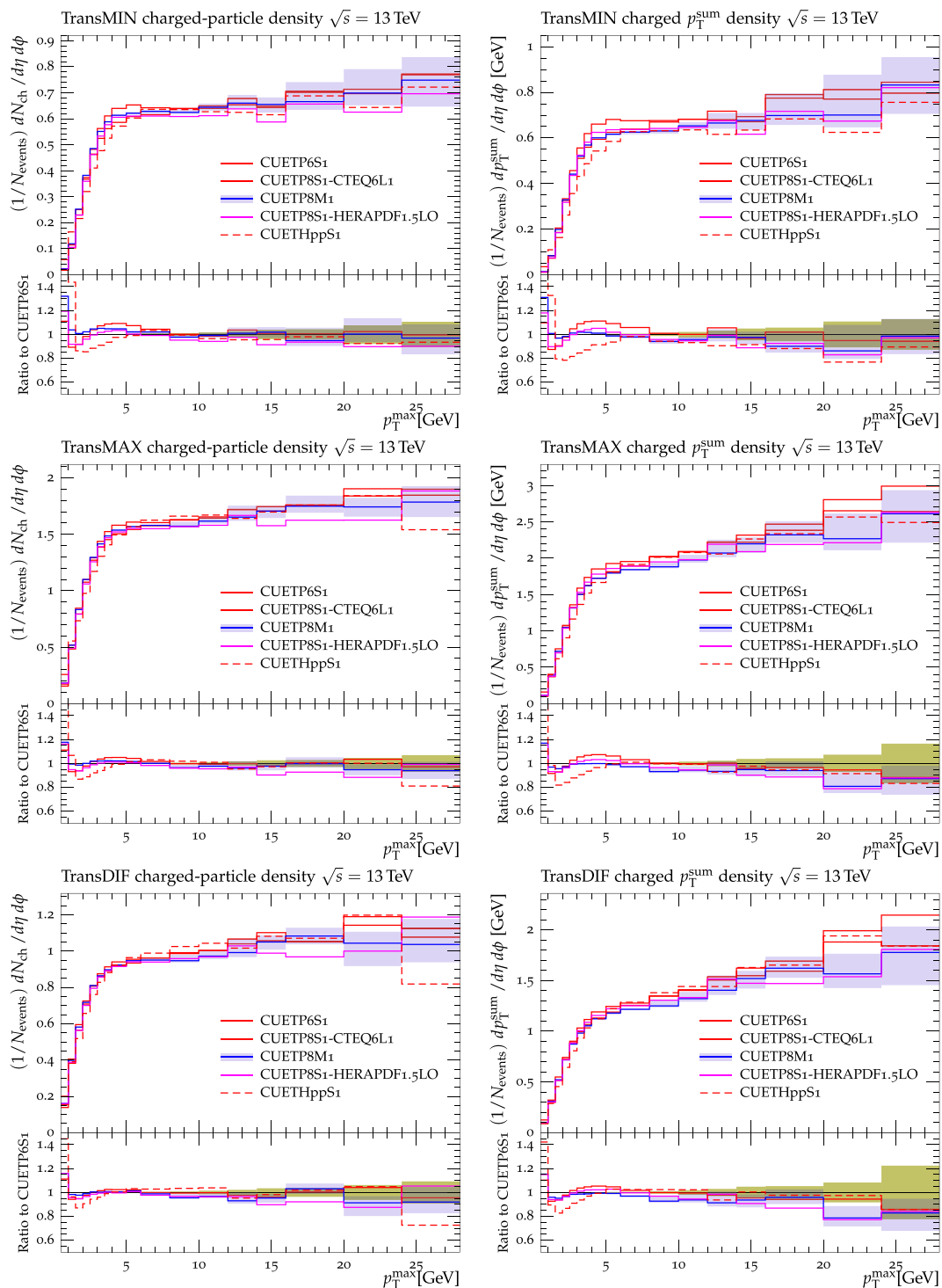
Fig. 19 Predictions at \sqrt{s} = 13 TeV for the particle (left) and the p_T^{\text{sum}} densities (right) for charged particles with p_T > 0.5 GeV and |\eta| < 0.8 in the TransMIN (top), TransMAX (middle), and TransDIF (bottom) regions, as defined by the leading charged particle, as a function of the leading charged-particle p_T^{\text{max}} for the five CMS UE tunes: PYTHIA6 CUETP6S1-CTEQ6L1, and PYTHIA8 CUETP8S1-
