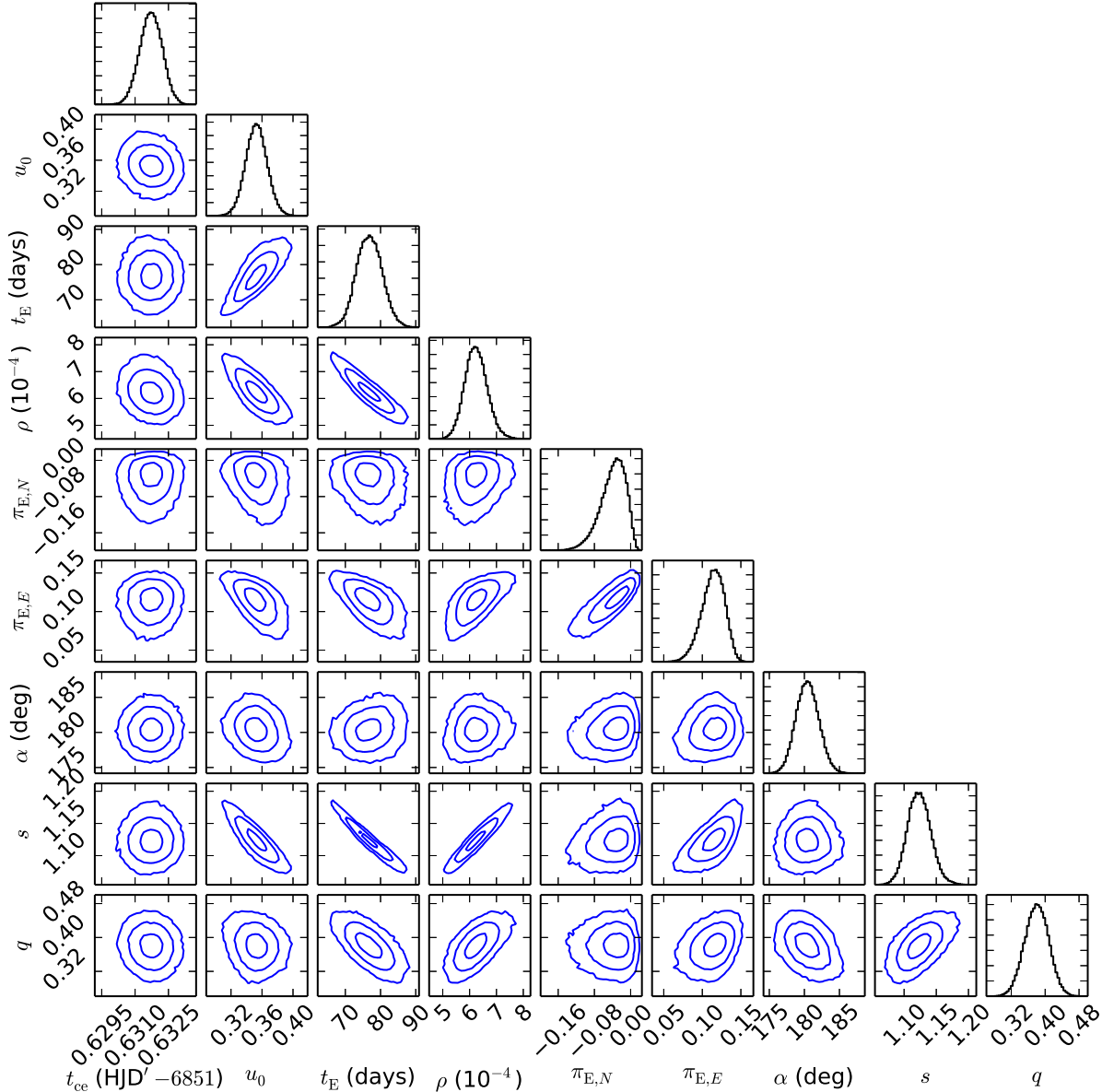
Figure 5. Full triangle diagram of the fitting parameters in the (+, +) solution without orbital motion. The contours (representing 1 \sigma , 2 \sigma , and 3 \sigma limits) enclose probabilities of 39%, 86%, and 99%, respectively.
