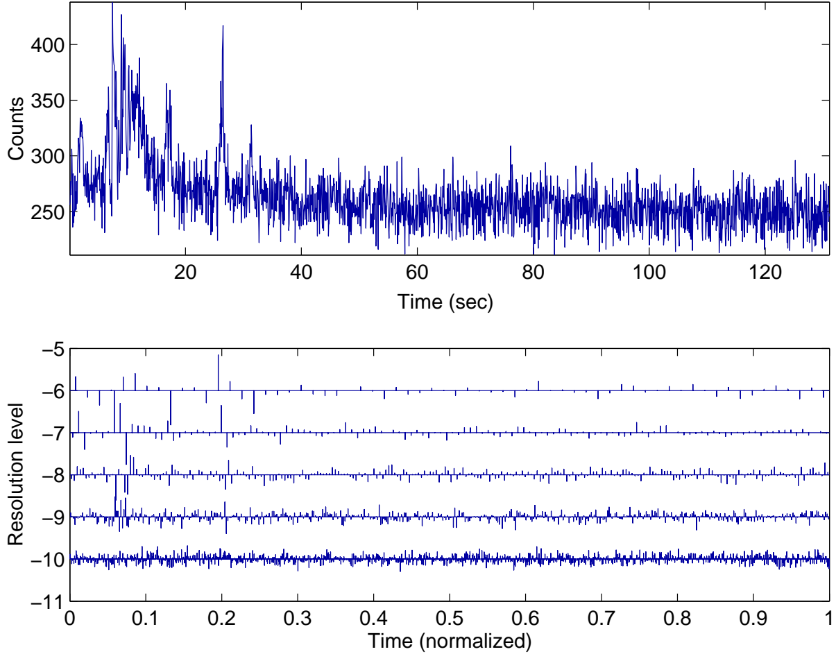
Fig. 1. Data from GRB990308 with z = 1.60 collected by BATSE trigger 7457 in a total number of 2^{11} 64 ms bins in the energy band 115-320 keV (top panel), and its Symmlet-10 (Mallat 1998) discrete wavelet transform (DWT) at the level L = 6 . The horizontal axis corresponds to the same time scale as in the original burst. Each level on the vertical axis shows the wavelet coefficients at a given resolution level (i.e., scale). The wavelet coefficients are represented by spikes whose size and direction (up or down) is determined by the magnitude and sign (+ or -) of the coefficient.
