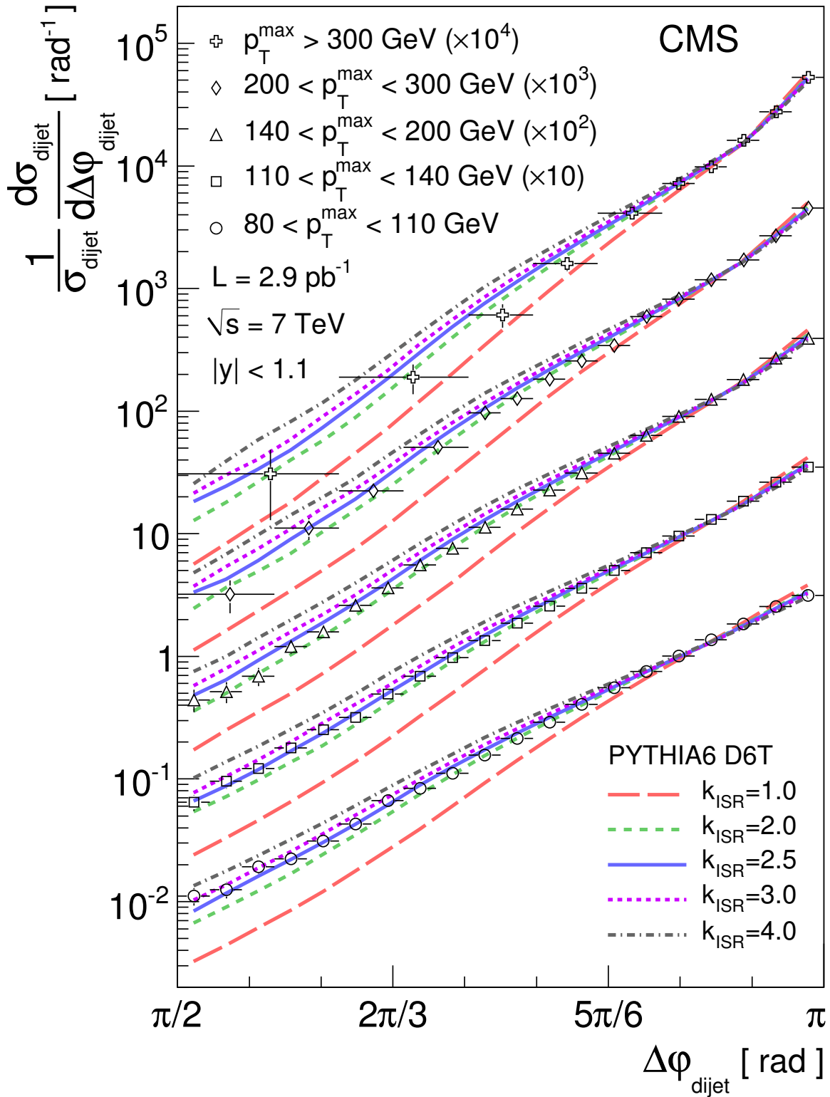
Figure 5: Normalized \Delta\phi_{\text{dijet}} distributions in several p_T^{\max} regions, scaled by the multiplicative factors given in the figure for easier presentation. The curves represent the predictions from PYTHIA6 with various values of k_{\text{ISR}} . The error bars on the data points include statistical and systematic uncertainties.
