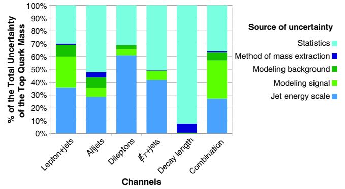
FIG. 5 (color online). The average uncertainties for CDF and D0 for each Run II measurement and for the Tevatron combination, separated according to major components. (See Table VIII in the Appendix for details on the systematic categories. In this figure, the jet and lepton modeling systematic uncertainties are grouped into the modeling background category.)
