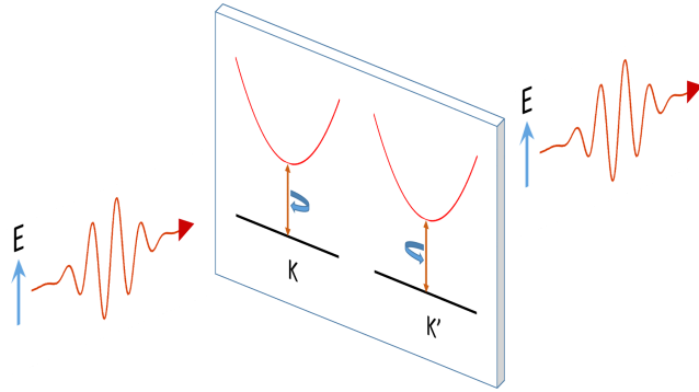
FIG. 1: (Color online) A sketch of excitons in K and K' valleys of MX 2 monolayers interacting with linearly polarized single photons. To ensure the interaction with one photon at a time, the power of incident radiation should not exceed \hbar\omega\Delta\omega , where \Delta\omega is the radiation bandwidth.
