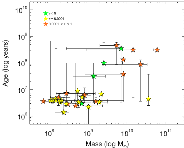
Figure 16. The distribution of \text{age}_{\text{SF}} versus mass for various \tau values for 33 LAEs. Green stars indicate models with exponentially increasing star formation rates ( \tau < 0 ), yellow stars are fits with a single instantaneous burst ( \tau_{\text{SF}} = 0.0001 Gyr), and orange stars are those with exponentially decaying star formation rates. Since mass and age parameters are correlated this plot is mainly meant to illustrate and confirm the distribution of \tau_{\text{SF}} with these parameters, showing that the oldest and most massive LAEs are those fit with increasing star formation rates, the youngest and least massive galaxies are fit with instantaneous star formation histories, and those LAEs with exponentially decaying star formation rates lie between those two populations.
