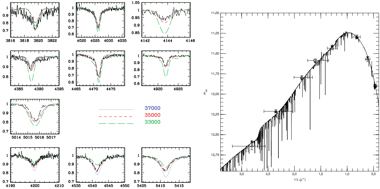
Figure 3. Left-hand panel: fit of the observed He lines (black solid line) by three CMFGEN models with T_{\text{eff}} = 33\,000\text{ K} (green long-dashed line), 35\,000\text{ K} (red short-dashed line) and 37\,000\text{ K} (blue dotted line). Right-hand panel: best SED (black solid curve) from the CHORIZOS run with fixed T_{\text{eff}} = 35\,000\text{ K} . The triangles with error bars are the photometric magnitudes used in the fit ( UBVIJHK ), the circle represents the measurement that was unused ( R ) and the stars are the synthetic magnitudes corresponding to the best SED.
