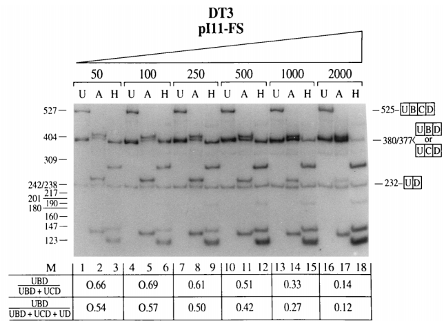
FIG. 7. DT3 cells contain a titratable factor or factors required for appropriate splicing regulation which can be overcome in transient transfections. Transient transfection of DT3 cells with increasing numbers of pI-11-FS minigenes resulted in stepwise loss of IIIb inclusion and increased IIIc inclusion, suggesting that a factor or factors required for regulation (i.e., IIIb inclusion and/or IIIc exclusion) is overwhelmed when large numbers of these minigenes are transfected. Abbreviations are defined in the legends to Fig. 2 and 3.
