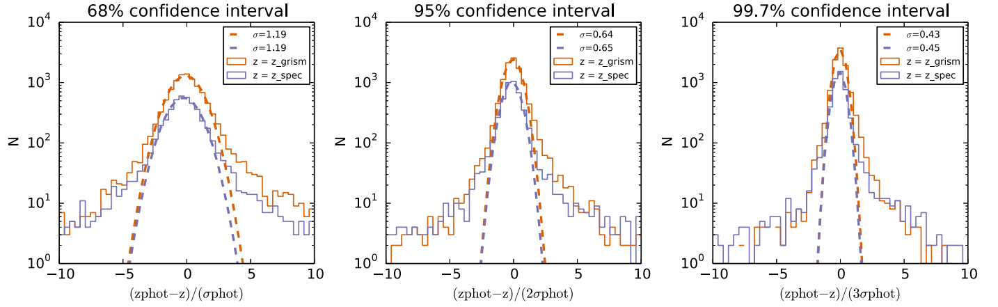
Figure 14. Redshift deviations normalized by 68%, 95%, and 99.7% confidence intervals for photometric redshifts (z_{\text{phot}} - z_{\text{true}})/(\sigma_{\text{phot}}) in the left panel, (z_{\text{phot}} - z_{\text{true}})/(2\sigma_{\text{phot}}) in the center panel, and (z_{\text{phot}} - z_{\text{true}})/(3\sigma_{\text{phot}}) in the right panel. Comparisons between photometric redshifts and spectroscopic redshifts (purple) or narrowed grism redshifts (orange) yield similar distribution shapes. Both exhibit roughly Gaussian distributions (fits are indicated with dashed lines) but \sigma \sim 1.2, 0.6, 0.4 suggesting that the redshift PDFs are narrower than the observed scatter in redshift by a factor of \sim 1.2 .
