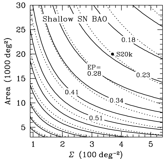
FIG. 2.—EP \sigma(w_p) \times \sigma(w_a) (solid lines) as a function of the survey area and SN surface density \Sigma (accumulated over 10 years). The EP contours are spaced logarithmically. The SN distribution is scaled from S20k (filled circle; 7.4 million SNe) by \Sigma . Photo- z parameters are the same as those of S20k, and the Planck priors are assumed. The total number of SNe is held constant along each dotted line, which is spaced at factors of \sqrt{2} .
