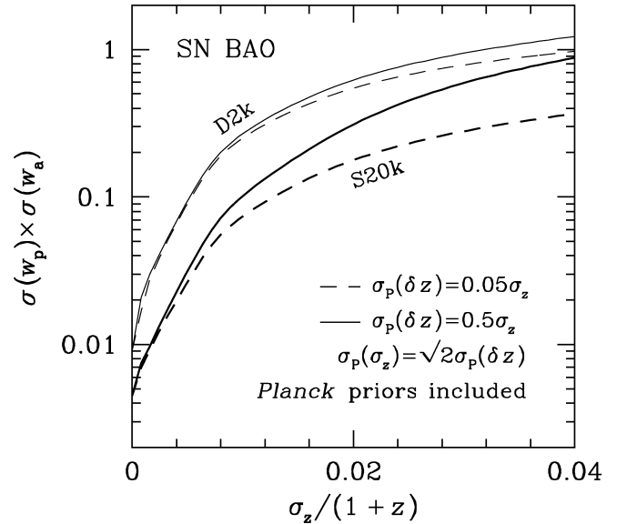
FIG. 1.—EP \sigma(w_p) \times \sigma(w_a) of S20k (thick lines) and D2k (thin lines) as a function of the rms photo- z error \sigma_z . The priors on the photo- z biases are taken to be 0.5\sigma_z (solid lines) and 0.05\sigma_z (dashed lines), which correspond to calibrations with 4 and 400 spectra per redshift bin, respectively, in the Gaussian case. To reduce the dimensions, we peg the prior on the photo- z rms to that on the photo- z bias: \sigma_p(\sigma_z) = \sqrt{2}\sigma_p(\delta z) . For comparison, LSST weak lensing, galaxy BAOS, and the two combined will achieve EP \sim 0.01, 0.02 , and 0.002 , respectively (Zhan 2006).
