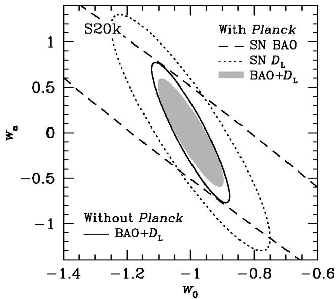
FIG. 3.—Marginalized 1\sigma error contours of the dark energy EOS parameters w_0 and w_a , from S20k SN BAOs (dashed line; EP = 0.22 with Planck ), luminosity distances (dotted line; EP = 0.064 with Planck ), and the two combined with (shaded area; EP = 0.012) and without (solid line; EP = 0.018) Planck .
