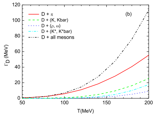
FIG. 1: (a) Total elastic cross sections for D - \pi (solid line), S -wave D - K (dashed line) and D - \rho (dash-dotted line) scattering based on the invariant amplitudes as discussed in the text; vertical lines indicate the respective thresholds. (b) Total D -meson scattering width in a meson gas (dash double dotted line), consisting of contributions from Goldstone bosons and vector mesons.
