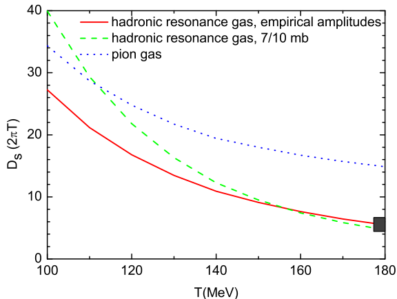
FIG. 5: Spatial D -meson diffusion coefficient in units of the medium’s thermal wavelength, 1/(2\pi T) . The filled box at the lower right indicates the range of values calculated for charm quarks in the QGP at 1.2T_c within an in-medium T -matrix approach [14].
