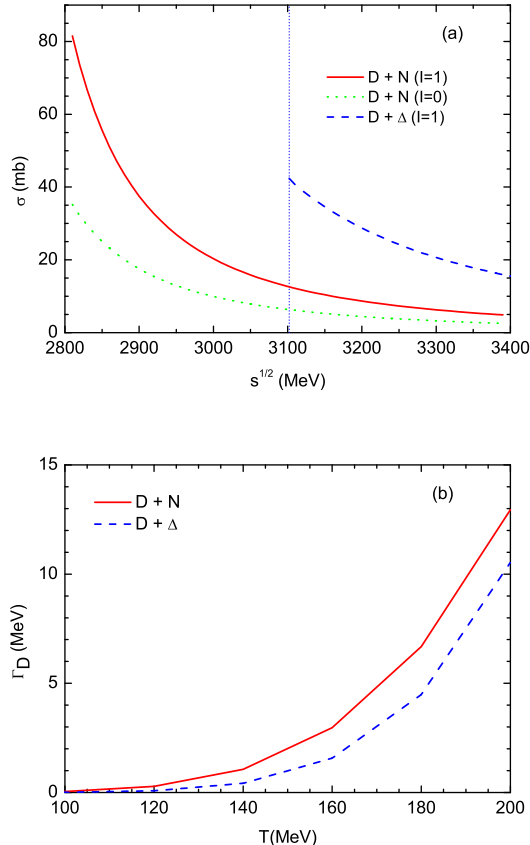
FIG. 2: (a) Elastic cross sections for S -wave D - N scattering in the I=1 (solid line) and I=0 (dotted line) channel, and D - \Delta scattering (dashed line, I=1 ; vertical line: D\Delta threshold) based on the invariant amplitudes as discussed in the text; (b) D -meson widths from D - N scattering (solid line, including both I = 1 and I = 0 channels) and from D - \Delta scattering (dashed line) at vanishing chemical potential.
