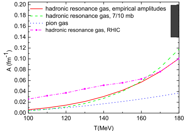
FIG. 4: Thermal relaxation rate of p_D=0.1 GeV D -mesons using empirical amplitudes in a hadron gas at vanishing (solid line) and finite (dash-dotted line with squares) chemical potentials, as well as in a pion gas (dotted line). The dashed line corresponds to isotropic D -meson cross sections with mesons (7 mb) and baryons (10 mb). The filled box at the upper right indicates charm-quark relaxation rates in a QGP at 1.2 T_c from in-medium T -matrix calculations [14].
