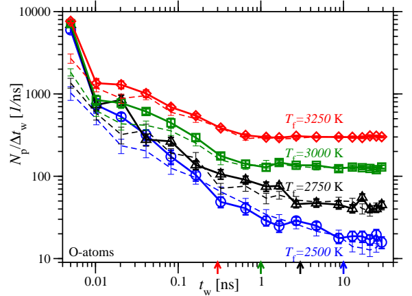
FIG. 2: (Color online) Number of jumping particles N_p per time \Delta t_w as function of waiting time t_w for the case of O-atoms and T_i = 5000 K (bold lines and symbols) and T_i = 3760 K (dashed thin lines). To be able to include on the logarithmic scale the data-point for the first time window at t_w = 0 , we plot \frac{N_p}{\Delta t_w}(t_w = 0) instead at t_w = 0.005 ns. For comparison the arrows indicate the equilibrium times t_{\text{eq}}^C ( t_{23} in [8]).
