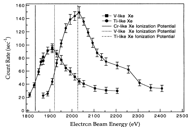
FIG. 4. Amplitudes of the 3d^4 5D_{2-5}D_3 observed titaniumlike and 3d^5 4G_{7/2-4}G_{9/2} vanadiumlike transitions in xenon versus electron beam energy, for 35 mA of electron beam current. The corresponding ionization energies are shown by vertical lines.
