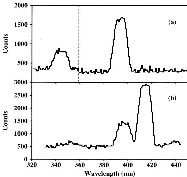
FIG. 1. Broad survey spectral scans with high (10 nm, monochromator slits removed) bandpass for (a) the 3d^4\ ^5D_2\text{-}^5D_3 transition in \text{Ba}^{+34} (right peak) and the 3d^5\ ^4G_{7/2}\text{-}^4G_{9/2} transition in \text{Ba}^{+33} (left peak), and (b) the corresponding transitions in \text{Xe}^{+32} and \text{Xe}^{+31} . The EBIT drift tubes were set at 2378 and 2277 V for the portions of the spectrum in (a) to the right and left of the dotted line, respectively, and at 2144 V for the entire spectrum in (b). The electron beam current was 50 mA throughout.
