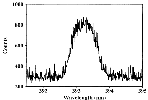
FIG. 2. 3d^4\ ^5D_2\text{-}^5D_3 transition in titaniumlike \text{Ba}^{+34} . The profile shown is the sum of 10 individual scans, each of which was accumulated in 5 min with a drift tube potential of 2378 V.
