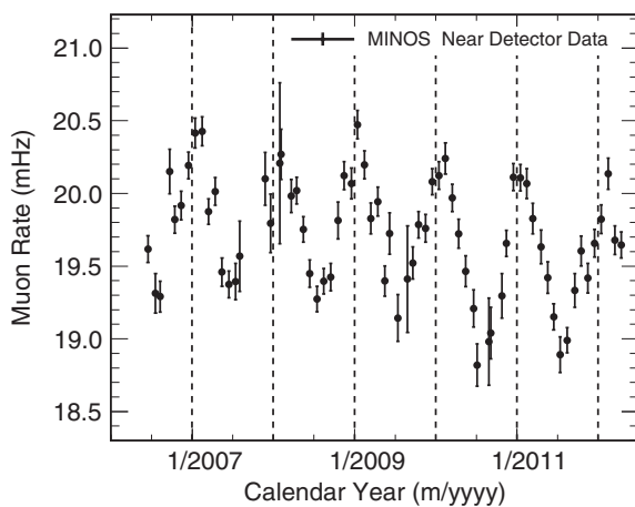
FIG. 6. The multiple-muon rate in the ND as a function of time. Each data point corresponds to one calendar month. A clear modulation in the data is observed with the maximum occurring towards the start of the year. The vertical lines are year boundaries.
