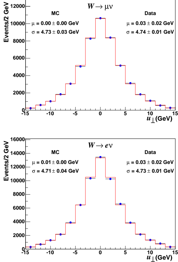
FIG. 43: The simulation (solid) and data (circles) u_{\perp} distributions for W boson decays to \mu\nu (top) and e\nu (bottom). The simulation uses parameters fit from Z boson data, and the uncertainty on the simulation is due to the statistical uncertainty on these parameters. The data mean ( \mu ) and RMS ( \sigma ) are well-modeled by the simulation.
