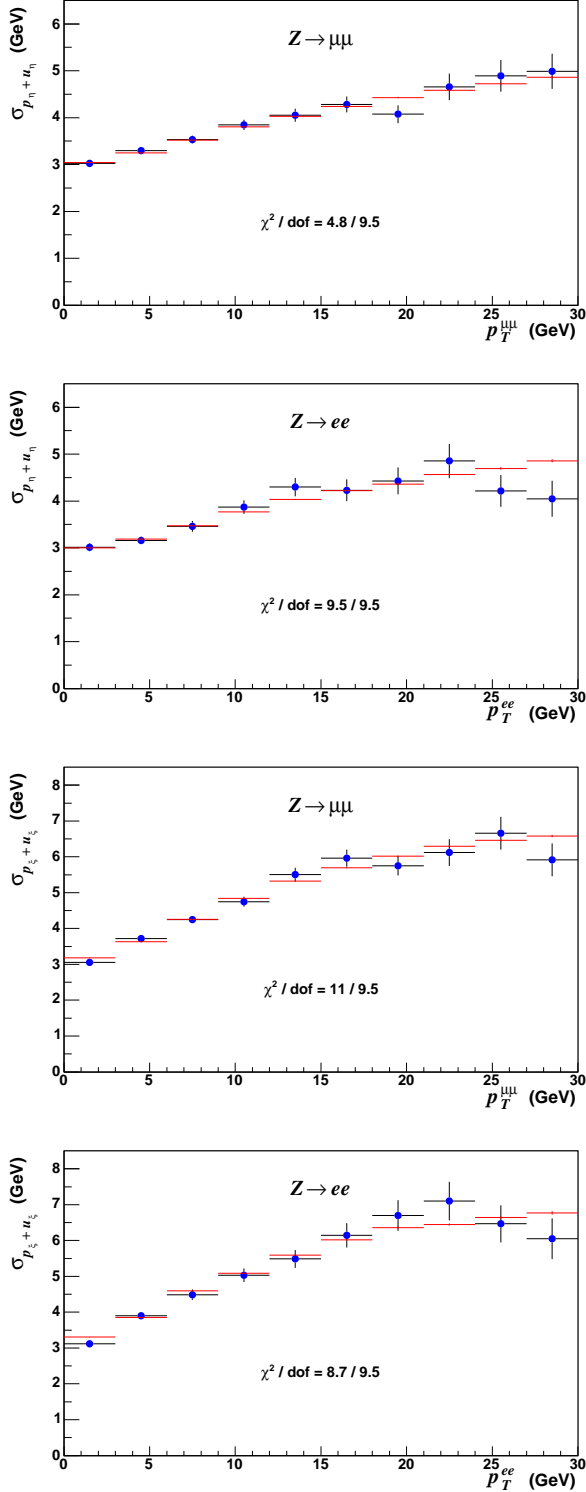
FIG. 41: The simulation (solid) and data (circles) p_T^{l1+l2} + u_\perp (top) and p_T^{l1+l2} + u_\xi (bottom) resolutions for Z boson decays to muons and electrons. The sum of the four \chi^2 values is minimized in the fit for the recoil resolution parameters N_{W,Z} and s_{hard} . Since there are four distributions and two fit parameters, each distribution contributes half a degree of freedom to the fit.
