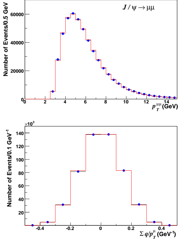
FIG. 21: The J/\psi \rightarrow \mu\mu data (points) and tuned simulation (histogram) distributions of p_T^{\mu\mu} (top) and \Sigma q/p_T^{\mu} (bottom). The \Sigma q/p_T^{\mu} is equal to the sum of the track curvatures of muons from a J/\psi decay, divided by 2.11593 \times 10^{-3} .
