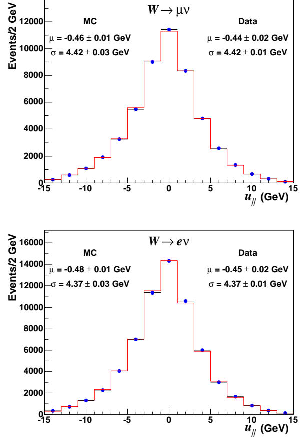
FIG. 42: The simulation (solid) and data (circles) u_\parallel distributions for W boson decays to \mu\nu (top) and e\nu (bottom). The simulation uses parameters fit from Z boson data, and the uncertainty on the simulation is due to the statistical uncertainty on these parameters. The data mean ( \mu ) and RMS ( \sigma ) are well-modeled by the simulation.
