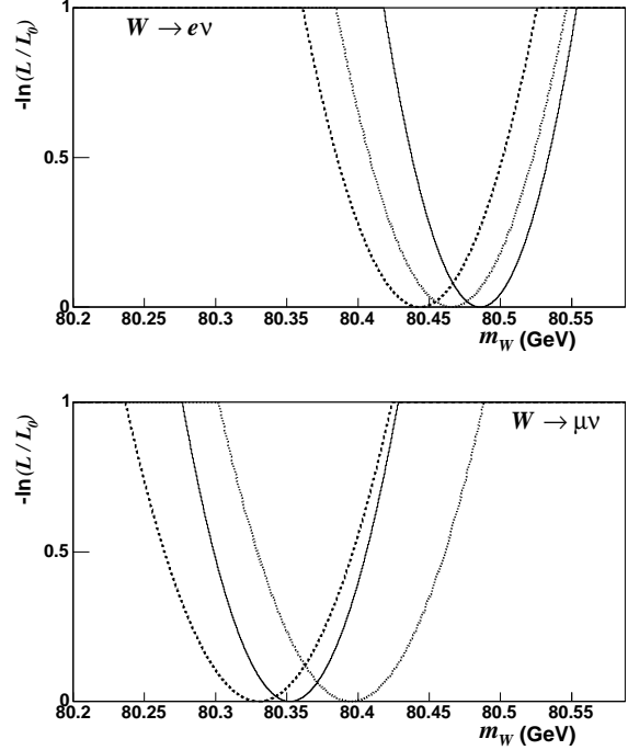
FIG. 54: The negative log of the likelihood ratio \mathcal{L}/\mathcal{L}_0 , where \mathcal{L}_0 is the maximum likelihood, as a function of m_W for the m_T (solid), p_T (dashed), and \cancel{p}_T (dotted) fits in the electron (top) and muon (bottom) channels.
