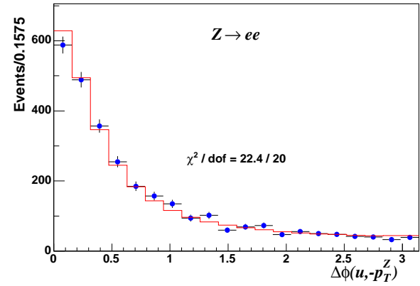
FIG. 40: The angle between the measured recoil and the direction opposite p_T^Z , for simulation (histogram) and data (circles) events where the Z boson decays to muons (top) or electrons (bottom). The \chi^2 from the Z \rightarrow \mu\mu sample is minimized in the fit to the recoil angular resolution. The corresponding uncertainty on m_W is negligible.
