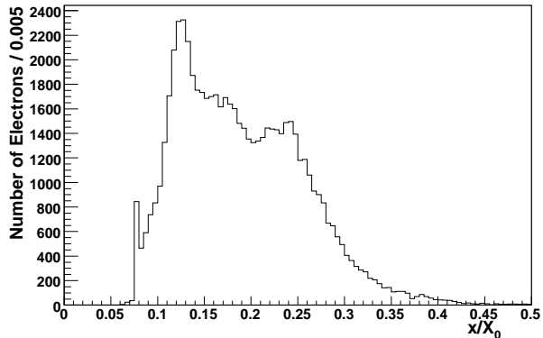
FIG. 9: The distribution of material upstream of the COT traversed by reconstructed electron trajectories in W \rightarrow e\nu data events, in units of radiation lengths. The peaks at \approx 0.08 , \approx 0.13 , and \approx 0.24 correspond respectively to trajectories outside the silicon detector ( |z| > 45 cm), within the silicon detector, and crossing silicon barrels ( |z| \approx 15, 45 cm). The mean of the distribution is 19%.
