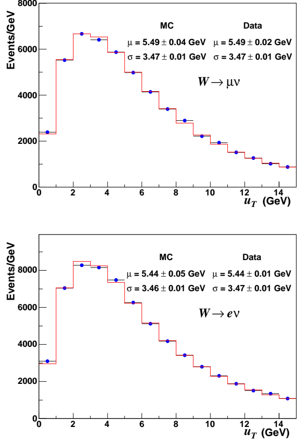
FIG. 44: The simulation (solid) and data (circles) u_T distributions for W boson decays to \mu\nu (top) and e\nu (bottom). The simulation uses parameters fit from Z boson data, and the uncertainty on the simulation is due to the statistical uncertainty on these parameters. The data mean ( \mu ) and RMS ( \sigma ) are well-modeled by the simulation.
