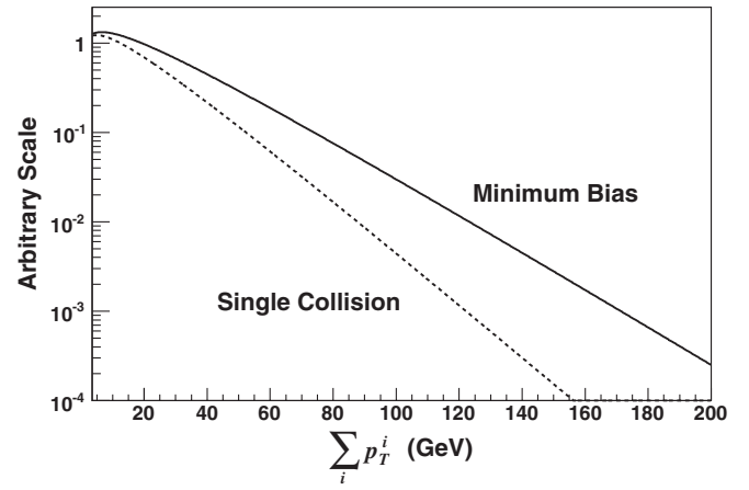
FIG. 39. The \sum_i p_T^i distribution for minimum bias data (solid line) and a single p\bar{p} collision (dashed line), as derived from the minimum bias distribution.
