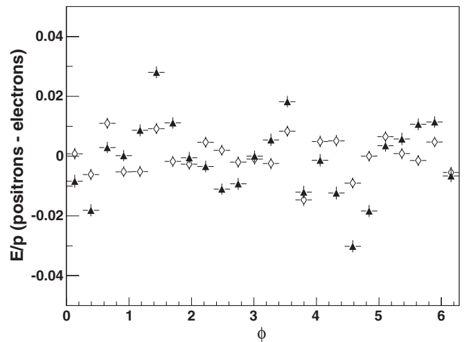
FIG. 20. The difference between e^+ and e^- E/p as a function of \cot\theta (top) and \phi (bottom) before (solid triangles) and after (open diamonds) track-level corrections.
