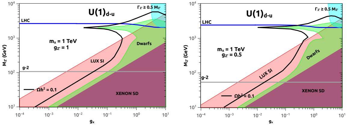
Figure 26. Same as in Fig. 6, for the U(1)_{d-u} model. Left: m_\chi = 1 TeV, g_{Z'} = 1 ; Right: m_\chi = 1 TeV, g_{Z'} = 0.5 .
