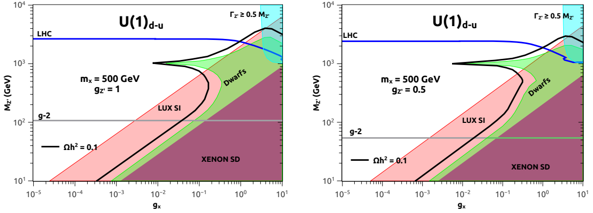
Figure 25. Same as in Fig. 6, for the U(1)_{d-u} model. Left: m_\chi = 500 GeV, g_{Z'} = 1 ; Right: m_\chi = 500 GeV, g_{Z'} = 0.5 .
