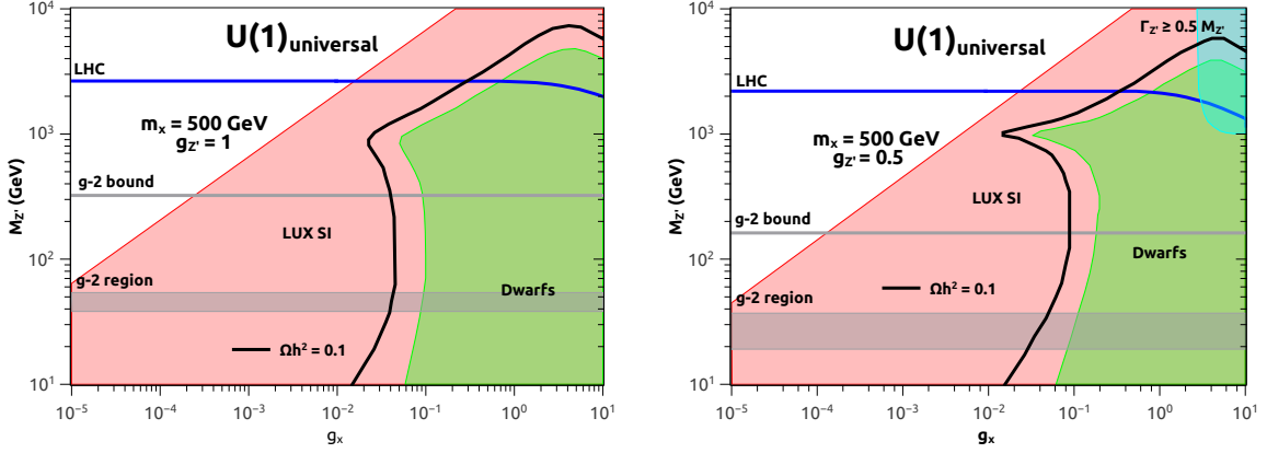
Figure 7. Same as in Fig. 6, for the U(1)_{\text{universal}} model. Left: m_\chi = 500 GeV, g_{Z'} = 1 ; Right: m_\chi = 500 GeV, g_{Z'} = 0.5 .
