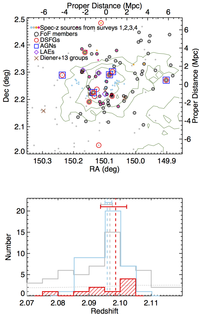
FIG. 2.— (Top) Spatial distributions of all spectroscopically confirmed galaxies at the redshift range of 2.07 < z \leq 2.12 from four redshift surveys (light blue dots: ZFIRE survey, orange dots: SPIRE/SCUBA 2 survey, gray dots: zCOSMOS survey, pink dots: MOSDEF/VUDS surveys). The right and top axes label the proper distance at z = 2.1 with respect to the cluster center. Black circles indicate sources that are linked to the ZFIRE cluster members with a linking length of 2 Mpc. Red circles show galaxies with L_{\text{IR}} \geq 10^{12} L_{\odot} , and blue boxes indicate X-ray sources. Purple diamonds show the positions of three LAEs from Chiang et al. (2015). Brown crosses mark the group candidates identified by Diener et al. (2013). Background dark green contours outline the z = 2.07 structure identified based on photometric redshifts ( \delta_{\text{gal}} = 0.2, 0.5, 0.8 from Figure 2 in Chiang et al. (2014)). (Bottom) Redshift distribution of the zCOSMOS SFGs (gray solid line), ZFIRE SFGs (sky blue solid line), and DSFGs (red shaded area) at 2.07 \leq z \leq 2.12 within a 10' radius from the ZFIRE cluster center. The dashed lines indicate the median redshifts of each sample, and the error bars represent the bootstrapped uncertainties. The gray dotted line represents the expected number of SFGs from the zCOSMOS survey.
