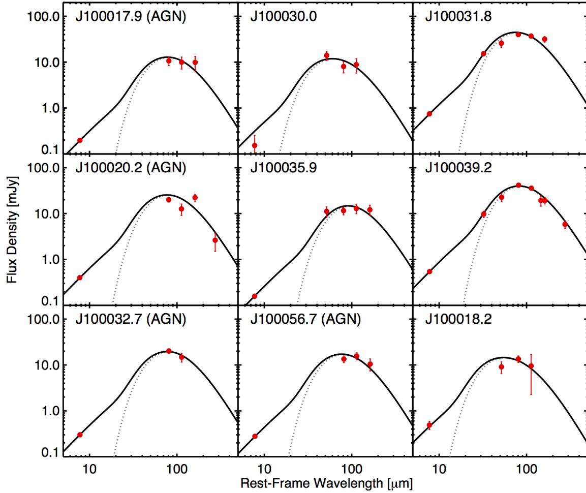
FIG. 1.— Rest-frame far-infrared SED of 9 DSFGs (including 4 X-ray luminous AGNs) within a 10' circle from the center of the ZFIRE cluster and a redshift range of 2.07 \leq z \leq 2.12 . The MIPS, PACS, SPIRE, and SCUBA 2 photometric data points and uncertainties are shown in red. The best-fit SED using a coupled graybody and mid-IR power law (Casey 2012) is shown in a black solid line, with the underlying graybody shown as a dotted line.
