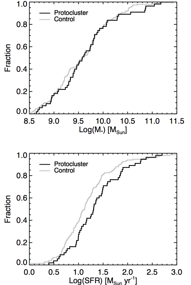
FIG. 3.— Normalized cumulative distributions of M_* (the top panel) and SFR (the bottom panel) of all SFGs from the zCOSMOS and SPIRE/SCUBA 2 surveys. The black solid lines show the distributions of SFGs that can be linked to the ZFIRE cluster and the gray solid lines show the distributions of the control sample.
