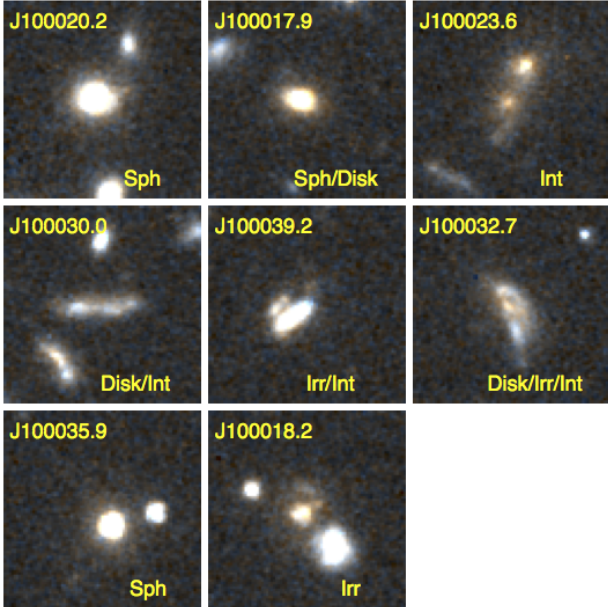
FIG. 4.— Three-color images of 8 DSFGs in the z \sim 2.1 structure with CANDELS WFC3 images available. WFC3 F125W, (F125W+F160W)/2 and, F160W used for the blue, green and, red channel, respectively. All images have the size of 5'' \times 5'' . The short name and morphology type of each DSFG are displayed in each panel. “Sph”, “Disk”, and “Irr” are shown when f_{\text{sph}} , f_{\text{disk}} , and f_{\text{irr}} are > 0.5 . DSFGs indicated as “Int” are candidates of mergers/interacting galaxies.
