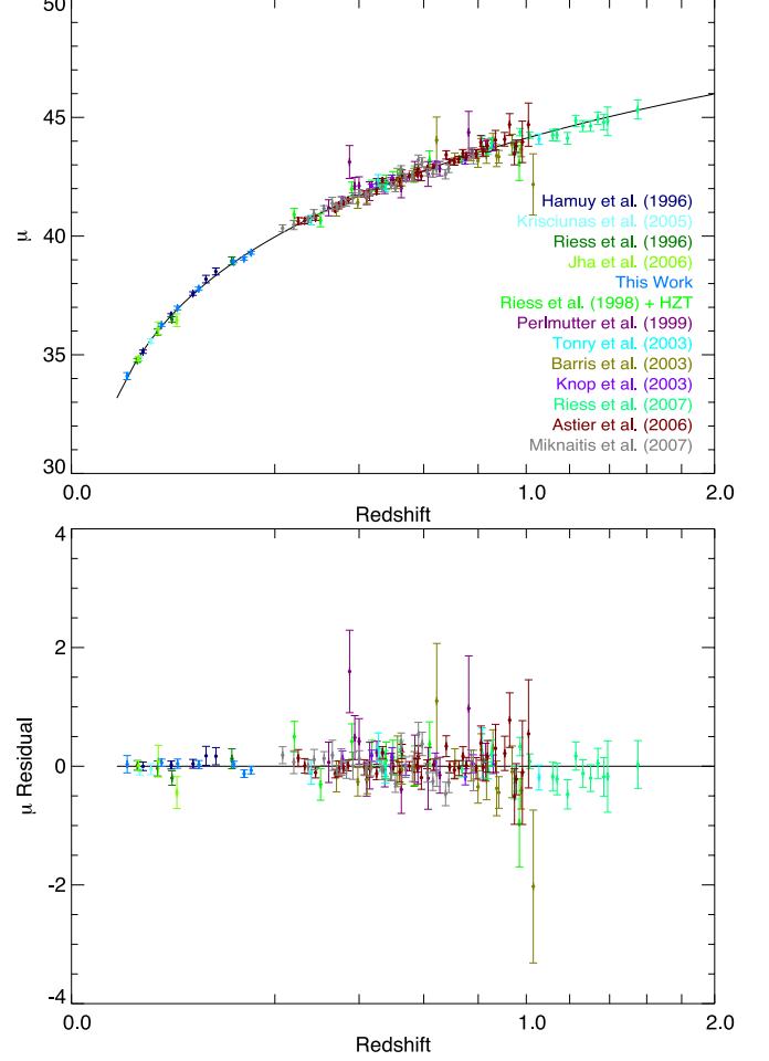
FIG. 10.— Top: Binned Hubble diagram (bin-size \Delta z = 0.01 ). Bottom: Binned residuals from the best fitting cosmology.
