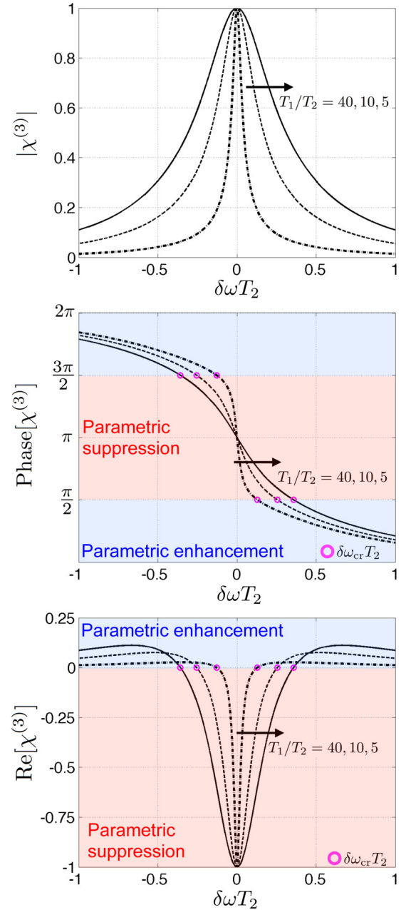
FIG. 7. The magnitude, phase, and real part of \chi^{(3)} are plotted vs \delta\omega T_2 for three different ratios T_1/T_2 = 40, 10, 5 . The parametric gain seen by the sidebands is determined by \text{Re}[\chi^{(3)}] . Low-frequency PPs lead to a parametric suppression of the gain. For the gain to be parametrically enhanced, \delta\omega must be large enough that the inversion can no longer follow the intensity in antiphase; in other words, the phase of \chi^{(3)} must be between -\pi/2 and \pi/2 .
