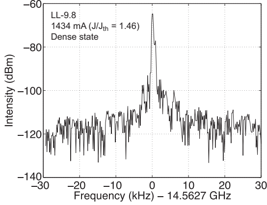
FIG. 10. The beat note of LL-9.8 at 1434 mA, the current at which the dense state appeared. The resolution bandwidth of the spectrum analyzer is 430 Hz.
