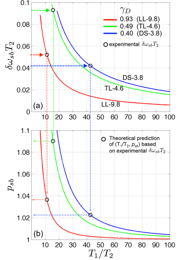
FIG. 12. Numerical solutions of the instability threshold obtained by setting the gain \bar{g} in Eq. (G38) equal to the loss \bar{\ell} , yielding both (a) the sideband separation \delta\omega_{\text{sb}}T_2 and (b) the pumping p_{\text{sb}} . The experimentally measured values of \delta\omega_{\text{sb}}T_2 are compared to the theory to infer T_1/T_2 , which also gives the theoretical prediction for the instability threshold p_{\text{sb}} .
