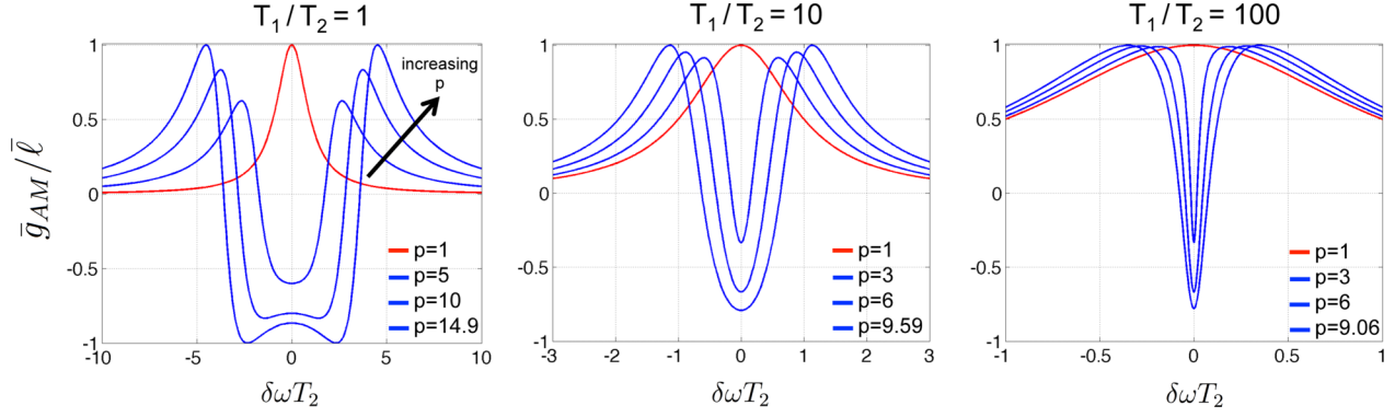
FIG. 11. The sideband gain \bar{g}_{AM}/\bar{\ell} of a traveling-wave laser, given in Eq. (G23), is plotted at various pump strengths, for three different values of T_1/T_2 : 1, 10, and 100. The largest value of p in each plot is equal to the instability threshold given in Eq. (G26).
