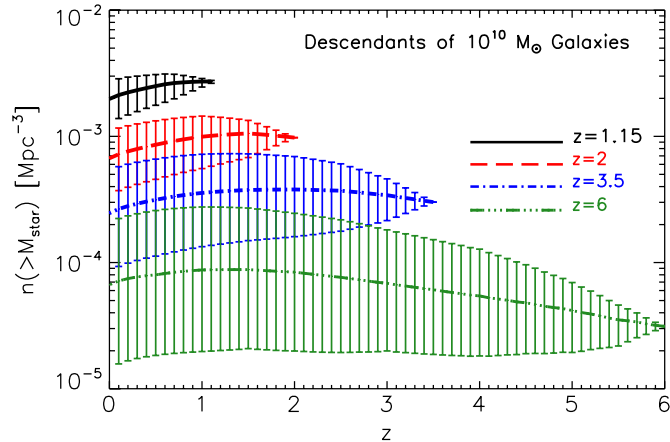
Figure 2. Evolution in median cumulative number density of the descendants of 10^{10} M_{\odot} galaxies at four separate starting redshifts ( z = 1.15, 2, 3.5, and 6 ). Contrast with the cumulative number density evolution of progenitors above. (A color version of this figure is available in the online journal.)
