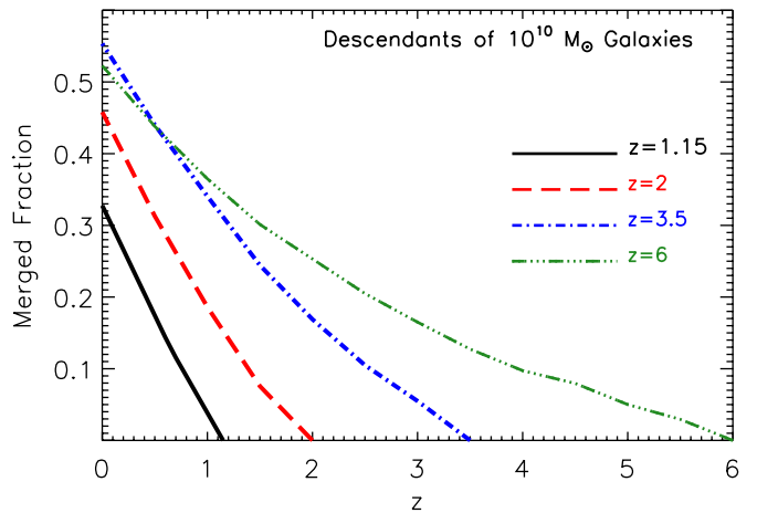
Figure 3. Fraction of descendants which have been lost due to mergers with a larger galaxy as a function of redshift, for 10^{10} M_{\odot} galaxies at four separate starting redshifts ( z = 1.15, 2, 3.5, and 6 ).
