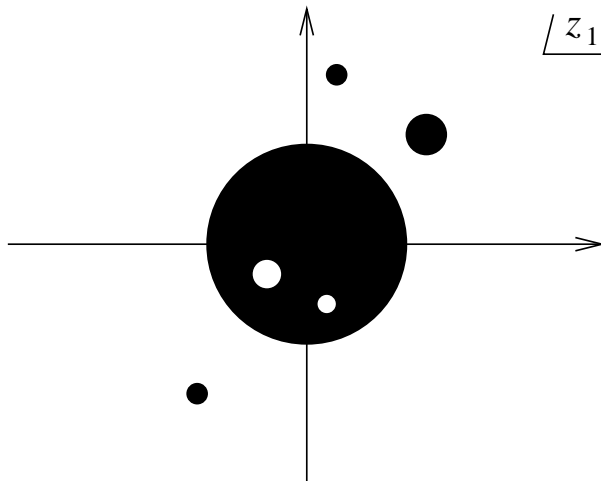
Figure 2: An LLM configuration with three droplets and two holes.
