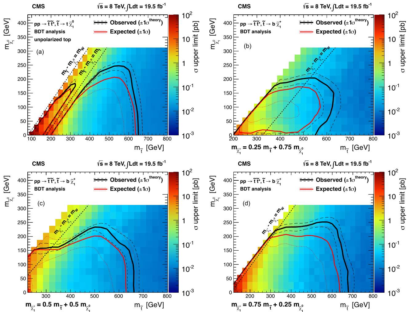
Fig. 10 Interpretations using the primary results from the BDT method. (a) \tilde{t} \rightarrow t \tilde{\chi}_1^0 model; (b) \tilde{t} \rightarrow b \tilde{\chi}_1^+ model with x = 0.25 ; (c) \tilde{t} \rightarrow b \tilde{\chi}_1^+ model with x = 0.50 ; (d) \tilde{t} \rightarrow b \tilde{\chi}_1^+ model with x = 0.75 ; The color scale indicates the observed cross section upper limit. The
