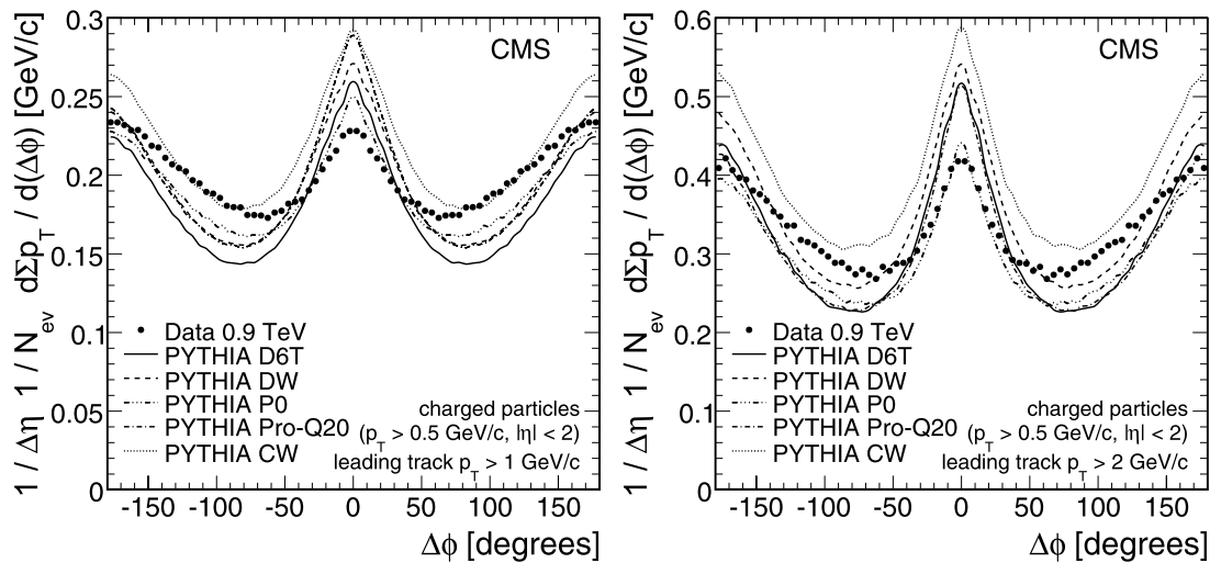
Fig. 2 Average scalar sum of transverse momenta of charged particles with p_T > 0.5 GeV/c and |\eta| < 2 , per unit of pseudorapidity and per radian, plotted as a function of the azimuthal angle difference \Delta\phi relative to the leading track (the measurements have been symmetrized in
