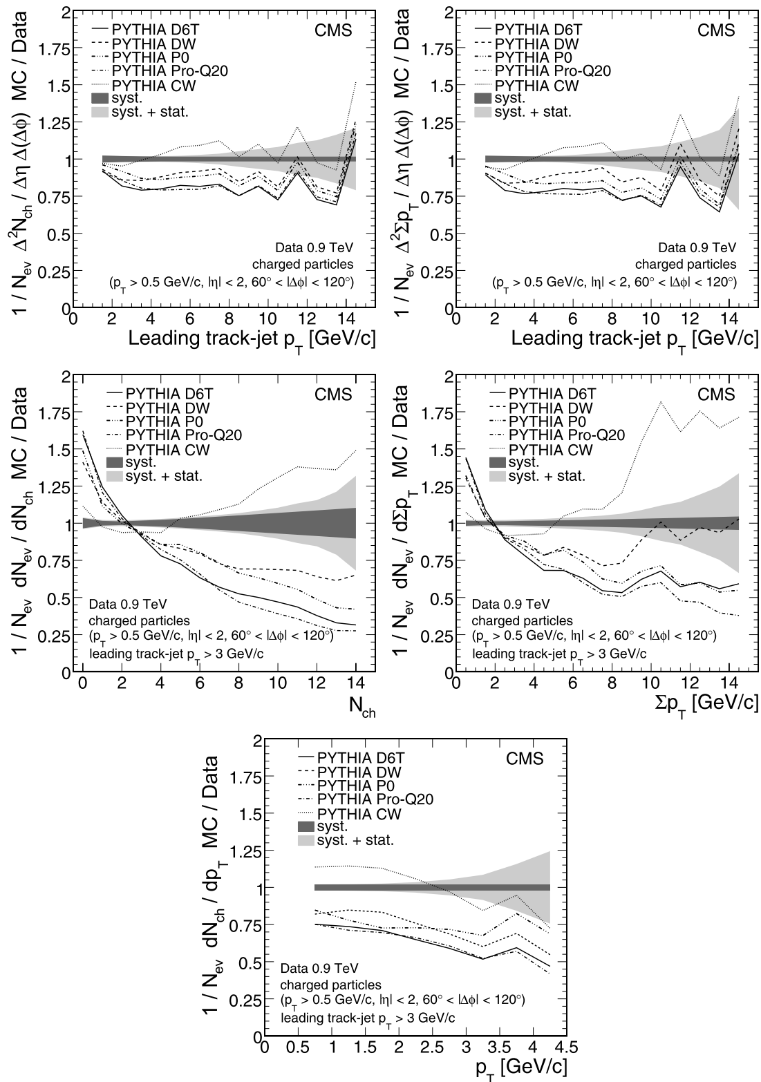
Fig. 5 Ratios of various MC predictions, including full detector simulation, to the measurements of hadrons with p_T > 0.5 GeV/c and |\eta| < 2 in the transverse region, 60^\circ < |\Delta\phi| < 120^\circ : (from top left to bottom) average multiplicity of charged particles, as a function of the leading track-jet p_T (cf. Fig. 3, upper right); average scalar \sum p_T , as a function of the leading track-jet p_T (cf. Fig. 3, lower right); dis-
