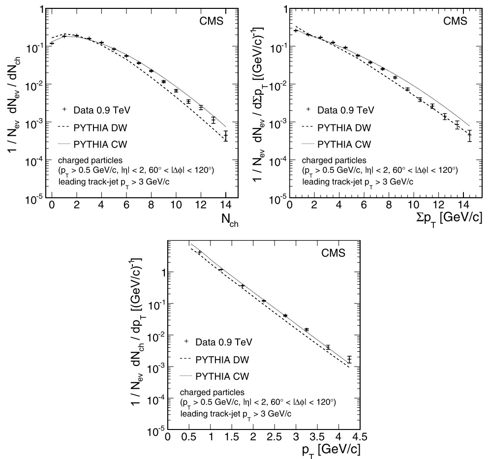
Fig. 4 For charged particles with p_T > 0.5 GeV/c and |\eta| < 2 in the transverse region, 60^\circ < |\Delta\phi| < 120^\circ : (upper left) multiplicity distribution; (upper right) scalar \sum p_T distribution; (bottom) p_T spectrum. The leading track-jet is required to have |\eta| < 2 and p_T > 3 GeV/c. The inner error bars indicate the statistical uncertainties affecting the measurements; for convenience systematic uncertainties on MC predictions are presented in the form of systematic uncertainties on the data points; the outer error bars thus represent the statistical uncertainties on the measurements and the systematic uncertainties affecting the MC predictions added in quadrature. Predictions of the DW and CW PYTHIA MC tunes, including full detector simulation, are compared to the data
