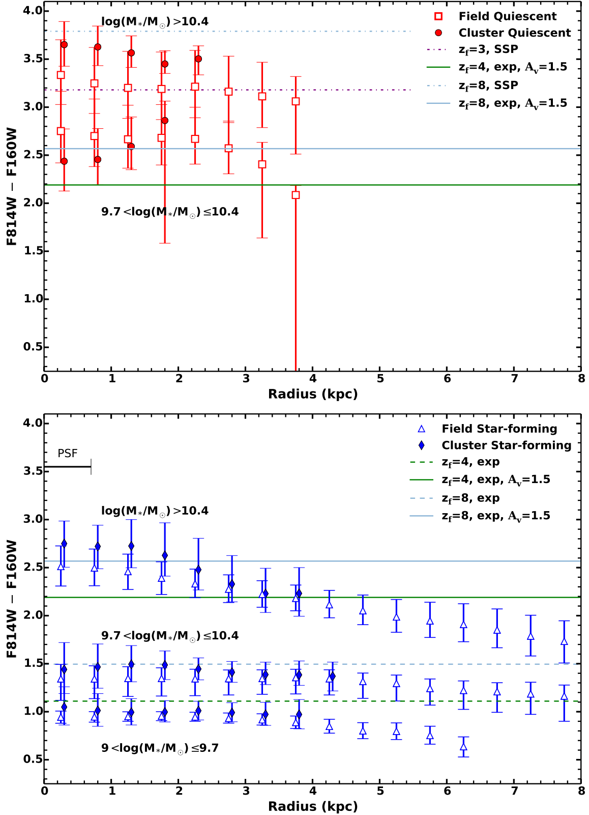
FIG. 7.— Observed radial color profiles for quiescent (top panel) and star-forming (bottom panel) field and cluster galaxies. Quiescent cluster (field) galaxies are shown as filled (open) red circles (squares). Star-forming cluster (field) galaxies are shown as filled (open) blue diamonds (triangles). In each panel our samples are separated by stellar mass. We show the extent of the HWHM of the HST /F160W PSF as a black line. The dashed lines are colors calculated using stellar population evolution models from EZGAL . Models with exponentially declining star-formation are labeled "exp" while models with a single stellar population are labeled "SSP". We find that stellar evolution models with no dust and solar metallicity are consistent with the low and intermediate mass star-forming sample. For the high mass star-forming sample, models with dust extinction of A_v = 1.5 are necessary to account for the redder colors. Single stellar population models are consistent with the colors we find for our high mass quiescent galaxy sample. However, the colors of the intermediate mass quiescent sample are consistent with exponentially decreasing star formation and a dust extinction of A_v = 1.5 .
