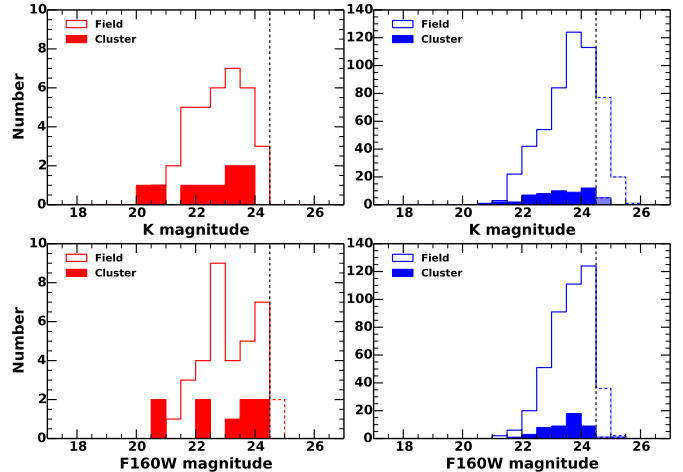
FIG. 3.— Top: Distributions of m_K for our sample of field (open histograms) and cluster (closed histograms) quiescent (left panel) and star-forming (right panel) galaxies. The dashed and light color histograms show where the field and cluster samples fall below the K-band magnitude limit of m_K > 24.5 AB mag (for \log(M_*/M_\odot) \geq 9 ) shown as a dashed black line. We remove galaxies that fall below this limit. Bottom: Distributions of m_{F160W} magnitudes for our sample of field (open histograms) and cluster (closed histograms) quiescent (left panel) and star-forming (right panel) galaxies. The dashed and light color histograms show where the field and cluster samples fall below the m_{F160W} magnitude limit for reliable sizes, shown as a dashed black line.
