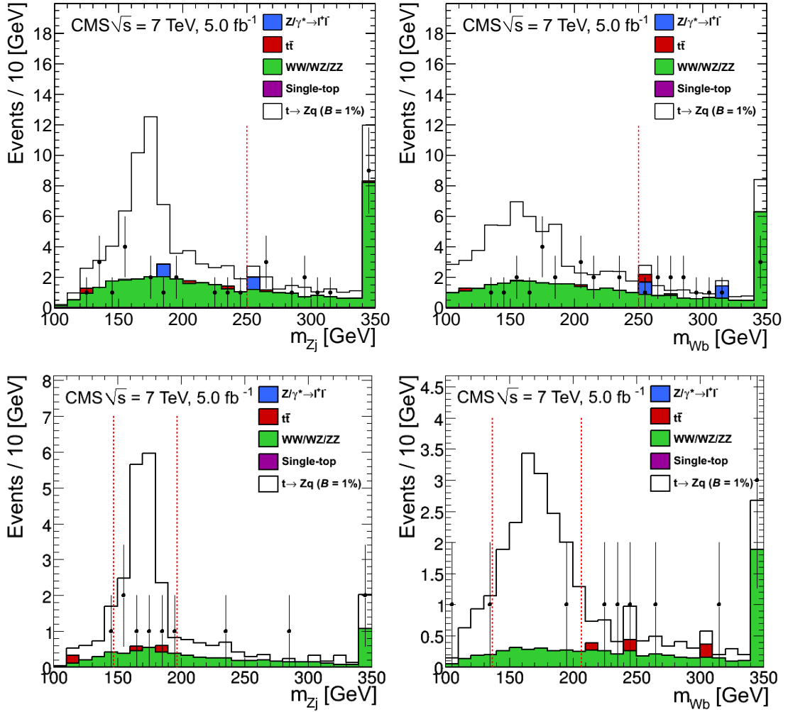
Figure 2: Comparison between data and simulated events of the m_{Zj} and m_{Wb} distributions after the basic event selection described in Section 3 for an integrated luminosity of 5.0 \text{ fb}^{-1} , requiring at least two jets and: (Top) the minimum S_T value, as required in the S_T selection; (Bottom) exactly one b jet as required in the b-tag based selection. The data are represented by the points with error bars and the open histogram is the expected signal assuming \mathcal{B}(t \rightarrow Zq) is equal to 1%. Stacked solid histograms represent the dominant backgrounds. The last bin contains all the overflow events. The red dotted lines show the boundaries of the allowed mass region.
