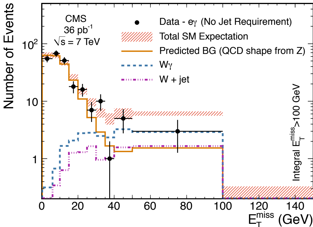
Figure 2: The E_T^{\text{miss}} distribution of the e\gamma candidates (solid circles with error bars) is compared to the QCD expectation for this spectrum from Z \rightarrow ee events (solid histogram). The W\gamma and W plus jet (with the jet misidentified as a photon) contributions are shown as dashed and dash-dotted histograms, respectively. The hatched red band represents the sum of all expected background components, and its width corresponds to the sum of the statistical and systematic uncertainties on the backgrounds.
