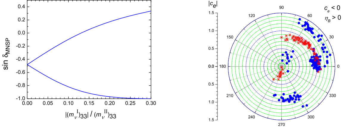
Figure 6: \sin \delta_{\text{MNSP}} is plotted as a function of the ratio of the type I contribution to the type II contribution ( |(m_{\nu}^{\text{I}})_{33}|/(m_{\nu}^{\text{II}})_{33} ) in the heaviest neutrino mass [Left]. The |c_e| is plotted as a function of \delta_{\text{MNSP}} for \eta_B > 0 and [Right] for v_R \simeq U_{14}(2/c_{\nu}) (1 - 2.5) \times 10^{15} \text{ GeV} .
