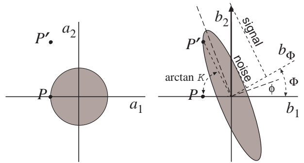
FIG. 7. Noise ellipses for a variational-output interferometer. Left : Noise for the ordinary vacuum that enters the interferometer’s dark port. Right : Noise for the field that exits the dark port along with the gravitational-wave signal. These noise ellipses are the same as for a conventional interferometer, Fig. 5, but here the quantity measured is the quadrature amplitude b_\Phi with frequency dependent phase \Phi \equiv \text{arccot} \mathcal{K} . It is informative to compare the measured phase \Phi with the angle of ponderomotive squeeze \phi = \frac{1}{2} \text{arccot}(\mathcal{K}/2) . They are related by \tan \Phi = \frac{1}{2} \tan 2\phi = \tan \phi / (1 - \tan^2 \phi) , so \Phi is always larger than \phi ; but for large \mathcal{K} (strong beating of the SQL), they become small and nearly equal.
