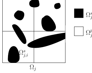
FIGURE 4.1. Subdomain with connected components of \Omega_j^s . In the present configuration L_j = 7 .
