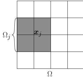
FIGURE 2.1. Triangulation \mathcal{T}_H .
