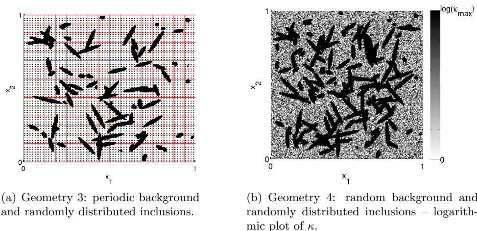
FIGURE 6.2. Two geometries with a 256 \times 256 fine mesh and a 16 \times 16 coarse mesh.
