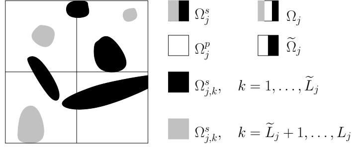
FIGURE 5.1. Subdomain with connected components of \Omega_j^s . The black connected components are those touching an edge interior to \Omega_j . The grey connected components are the remaining ones. In this configuration \tilde{L}_j = 4 and L_j = 7 .
