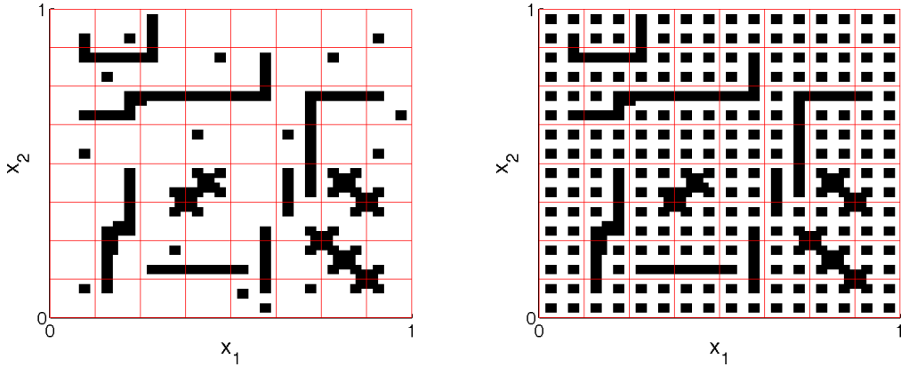
FIGURE 6.1. Two sample geometries: Geometry 1 (left) and Geometry 2 (right); the regions of low (white) and high (black) values of the coefficients. The mesh indicates the coarse triangulation.
