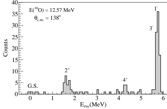
FIG. 3. ^{20}\text{Ne} excitation energy reconstructed from deuterons from the ^6\text{Li}(^{16}\text{O},d) reaction at \theta_{c.m.}=138^\circ . The energy of ^{16}\text{O} beam in the middle of the target is 12.57 MeV.
