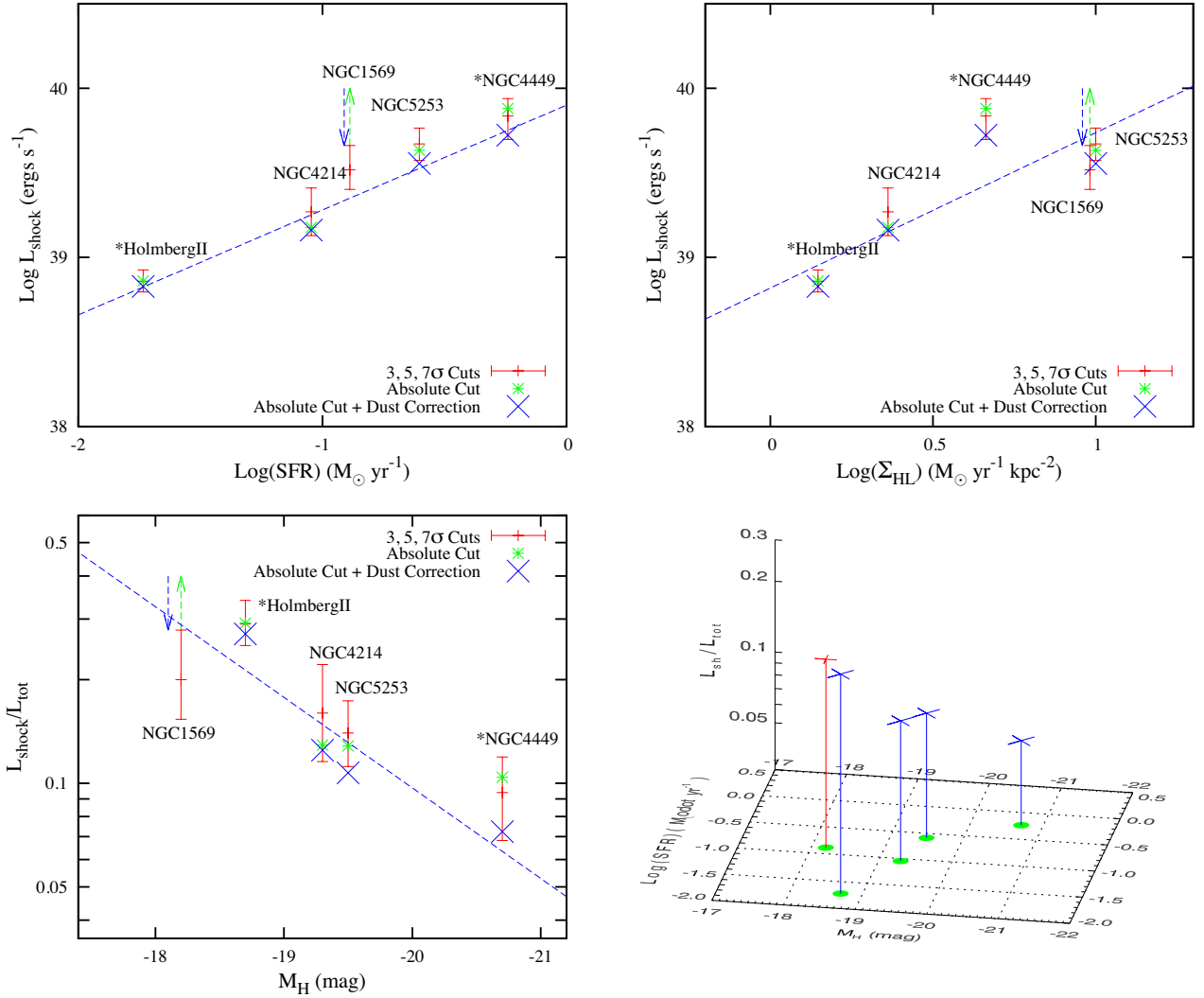
FIG. 13.— Corrections to L_{\text{shock}} : apparent thresholds, 3\sigma , 5\sigma , and 7\sigma (red bar), absolute threshold (green point), and dust correction to the line ratios (blue point). The dashed lines represent L_{\text{shock}} \propto \text{SFR}^{0.62 \pm 0.05} , L_{\text{shock}} \propto \Sigma_{\text{SFR,HL}}^{0.92 \pm 0.41} , and L_{\text{shock}}/L_{\text{tot}} \propto 10^{0.26(\pm 0.08)M_{\text{H}}} (or \propto (L_{\text{H}}/L_{\text{H},\odot})^{-0.65 \pm 0.2} ). Holmberg II and NGC 4449 are marked with asterisk (*) to indicate their uses of the [N II] diagnostics, while the others of the [S II] diagnostics. From the red bars, we can find that non-negligible amount of shocks can be found from a deeper observation. NGC 1569 is indicated as an arrow because the absolute cut corresponds to 1 – 2 sigma levels for the line emission images. Due to the heavy dust extinctions of NGC 1569, the dust correction should be significant for NGC 1569. We mark the dust correction effect as a blue arrow, which works in the opposite direction of the absolute cut effect. NGC 4449 and NGC 5253 turn out to have significant dust corrections (see the green and blue points). Though we have limited number statistics, this figure shows a strong evidence for the existence of regulations between the four quantities, L_{\text{shock}} , L_{\text{shock}}/L_{\text{tot}} , SFR, and M_{\text{H}} . The bottom-right panel shows the three dimensional plot of L_{\text{shock}}/L_{\text{tot}} vs. M_{\text{H}} and SFR. The four blue points are the same blue points on the other panels for NGC 4449, NGC 5253, NGC 4214, and Holmberg II. NGC 1569 is plotted in red with its 5\sigma cut result. The sub-linear scaling of L_{\text{shock}} \propto \text{SFR}^{0.62 \pm 0.05} can be due to projection effects of the three dimensional relation.
