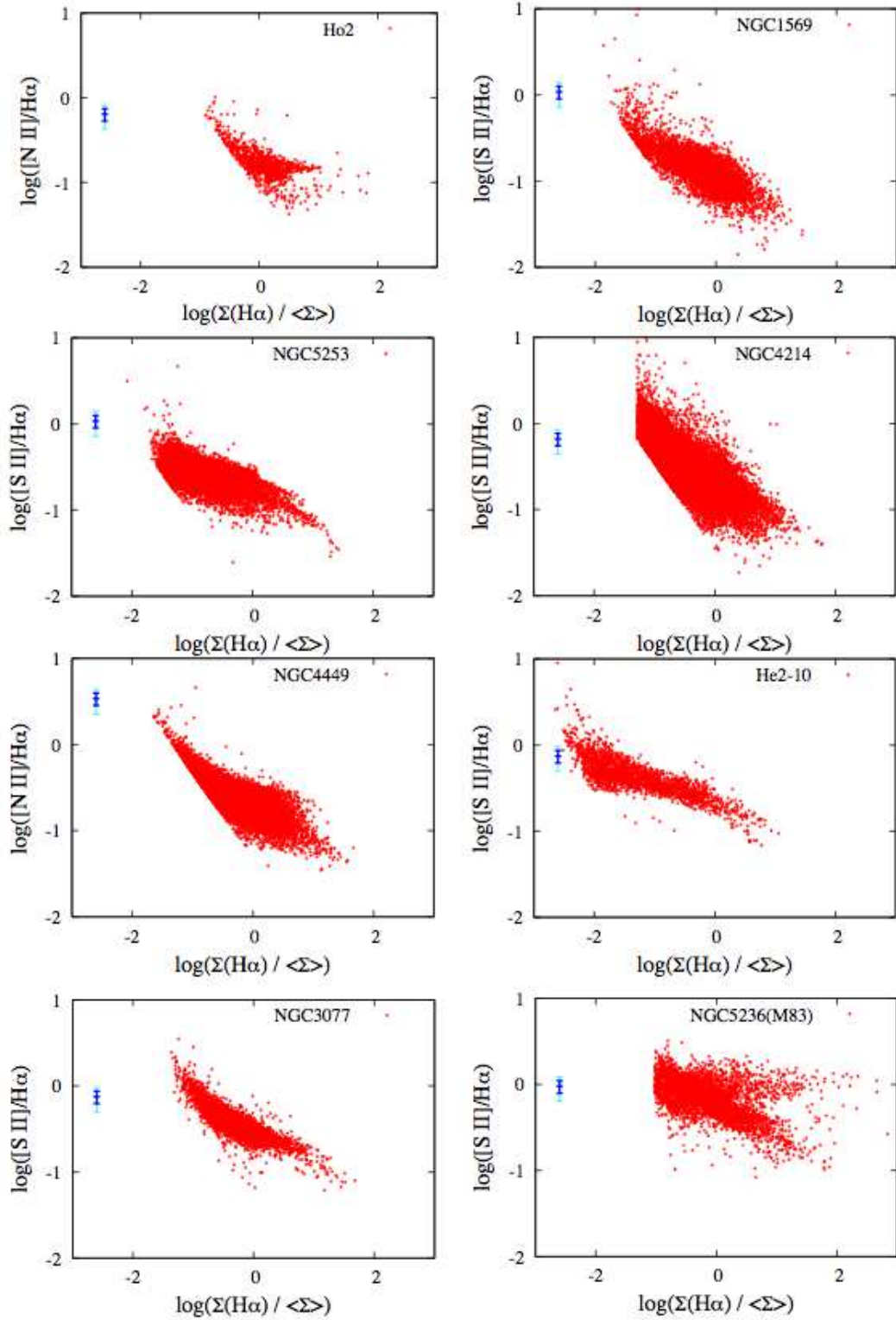
FIG. 9.— The line ratio of [S\ II](\lambda\lambda 6716, 6731)/H\alpha (and [N\ II](\lambda 6583)/H\alpha for Holmberg II and NGC 4449) as a function of the normalized H\alpha surface brightness with the error bars presented in Figure 5. We can use this ratio for shock separation, such as \log([S\ II](\lambda\lambda 6716, 6731)/H\alpha) > -0.5 , though the estimated shock is less reliable than the estimates from the diagnostic diagrams, because of the potential contamination from hot, diffuse photo-ionized gas.
