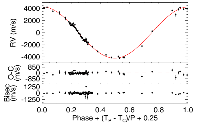
Figure 3. Points with uncertainties show the measured RVs for KELT-1 relative to the barycentric velocity of the system, phased to the best-fit period as determined from the model fit shown in the solid line (see Section 5.2). The phases are normally referenced to the time of periastron ( T_P ), but have been shifted such that a phase of 0.25 corresponds to the time of inferior conjunction T_C or transit. RV data near this phase show deviations from the Keplerian expectation due to the RM effect, which was included in the model. Middle panel: the residuals of the RV data from the model fit. Bottom panel: bisector spans as a function of phase.
