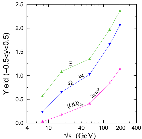
FIG. 3. Energy dependence of \Xi^- , \Omega^- , and (\Omega\Omega)_{0+} at midrapidity |y| < 0.5 for heavy ion collisions at an impact parameter of b \leq 3 fm in the AMPT model.
