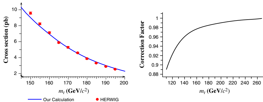
FIG. 8 (color online). Left: Cross section obtained from our normalization calculation as a function of m_t compared with the cross section used in HERWIG. Right: Normalization correction factor due to effective propagators as a function of m_t .
