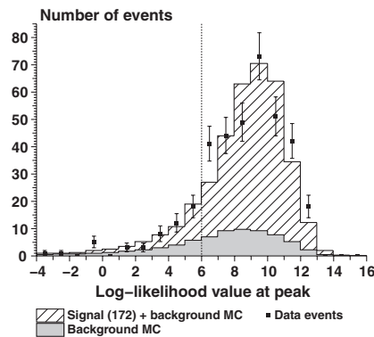
FIG. 15. Left: Measured 2-D likelihood on the data events. The plot shows the contours corresponding to a 1- \sigma , 2- \sigma , and 3- \sigma uncertainty (assuming Gaussian behavior) in our measurement. The marker shows the point of maximum likelihood. Right: Likelihood peak position of the individual likelihood curves for data and MC events. The dashed line indicates the likelihood cut of 6 employed.
