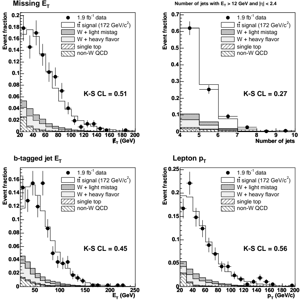
FIG. 3: Comparison of data and MC predictions for the selected events. The confidence level obtained from a K-S test on the two distributions is indicated on the histogram. The plots show, in order, the event \cancel{E}_T , the total number of jets with E_T > 12 GeV and |\eta| < 2.4 in the event, the E_T for all jets with a b -tag, and the lepton p_T .
