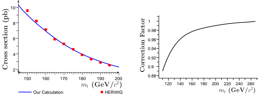
FIG. 8: Left: Cross section obtained from our normalization calculation as a function of m_t compared with the cross section used in HERWIG. Right: Normalization correction factor due to effective propagators as a function of m_t .
