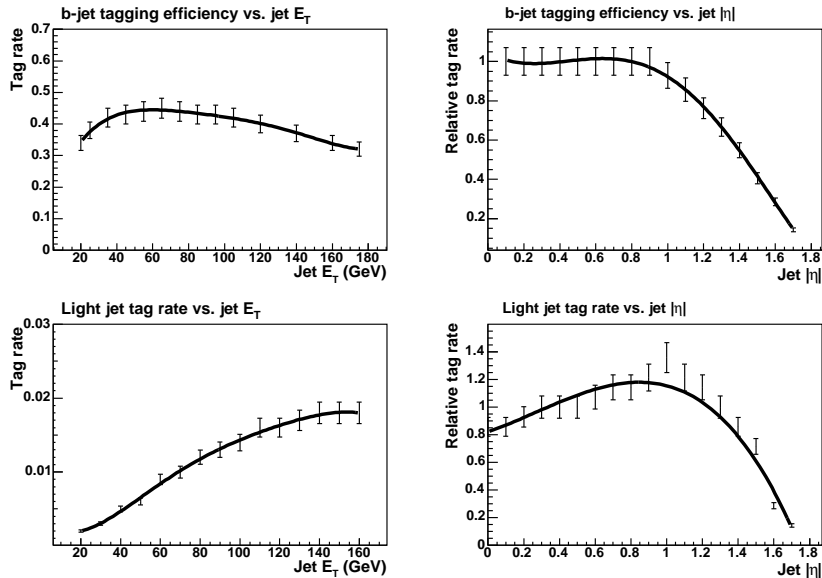
FIG. 4: Efficiency for the SECVTX algorithm with systematic uncertainties. The top two plots show the tag efficiency for tagging b -jets as a function of the jet E_T (left) and |\eta| (right), and the bottom two plots show the tag rate for light jets (mistags), also as a function of jet E_T (left) and |\eta| (right). The fits used as a parameterization in our analysis are also shown.
