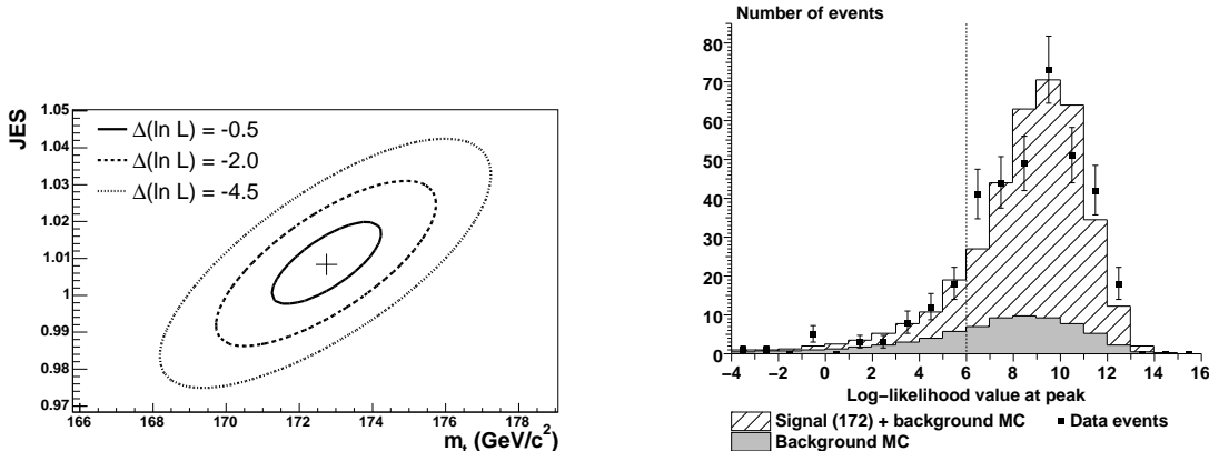
FIG. 15: Left: Measured 2-D likelihood on the data events. The plot shows the contours corresponding to a 1\text{-}\sigma , 2\text{-}\sigma , and 3\text{-}\sigma uncertainty (assuming Gaussian behavior) in our measurement. The calibration derived from MC events has been applied to both axes. The marker shows the point of maximum likelihood. Right: Likelihood peak position of the individual likelihood curves for data and MC events. The dashed line indicates the likelihood cut of 6 employed.
