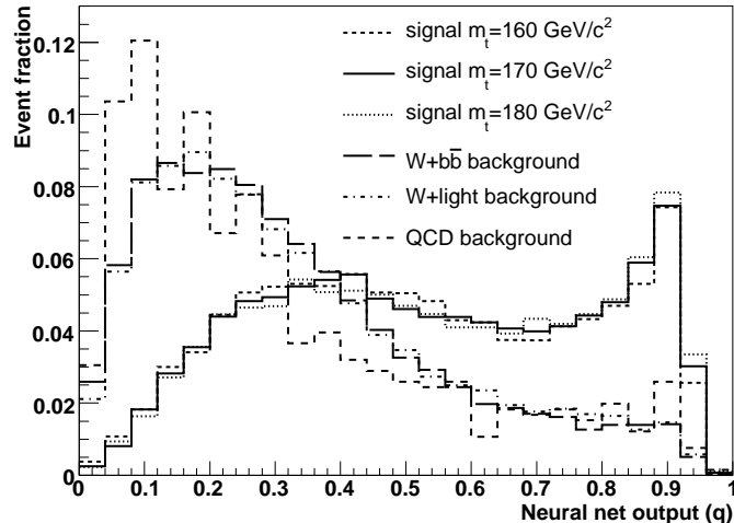
FIG. 10: The distributions of our neural network discriminant variable for signal and background MC events. The peaks on the right are from t\bar{t} signal events at three top masses. The peaks on the left are from various types of backgrounds.
