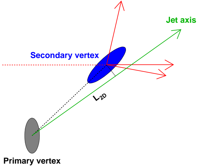
FIG. 1: A view of a b -jet in the x - y plane. L_{2D} , the distance between the primary and secondary vertices projected onto the jet axis, along with its uncertainty, is used to determine whether a jet originates from a heavy flavor quark.
