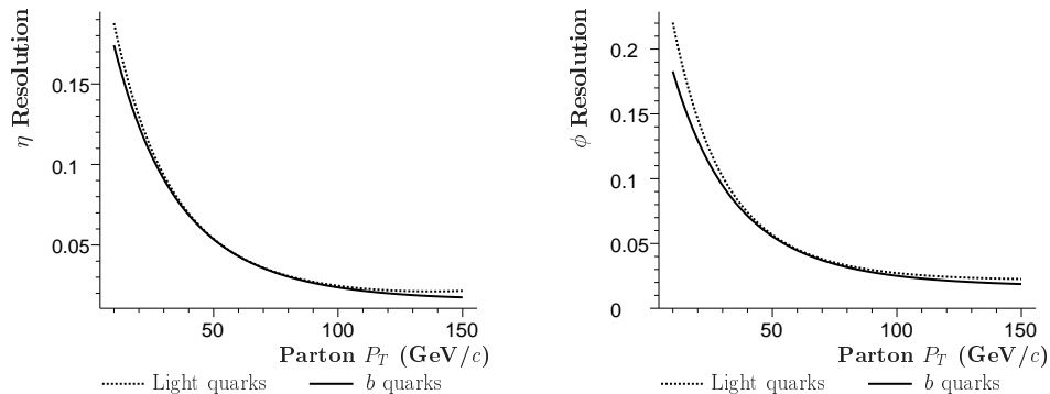
FIG. 5: Angular resolution in \eta (left) and \phi (right) as a function of parton p_T . The dashed line indicates the resolution for light quarks, and the solid line for b quarks.
