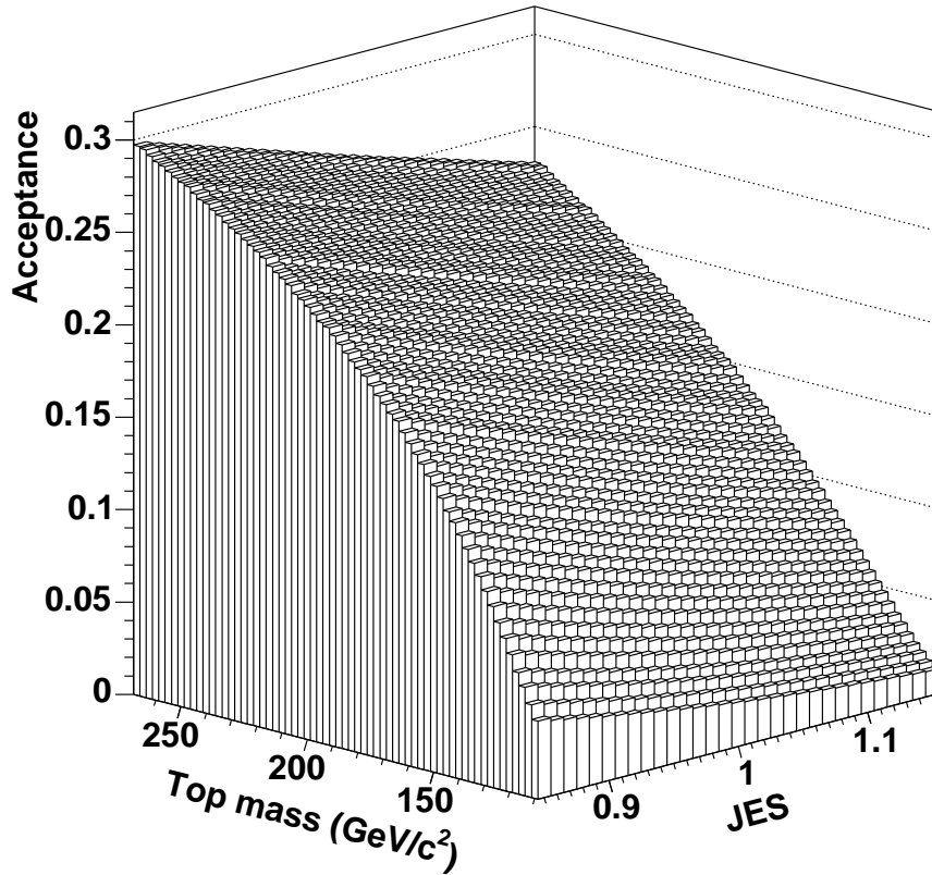
FIG. 9: Acceptance used in the integration as a function of m_t and JES.
