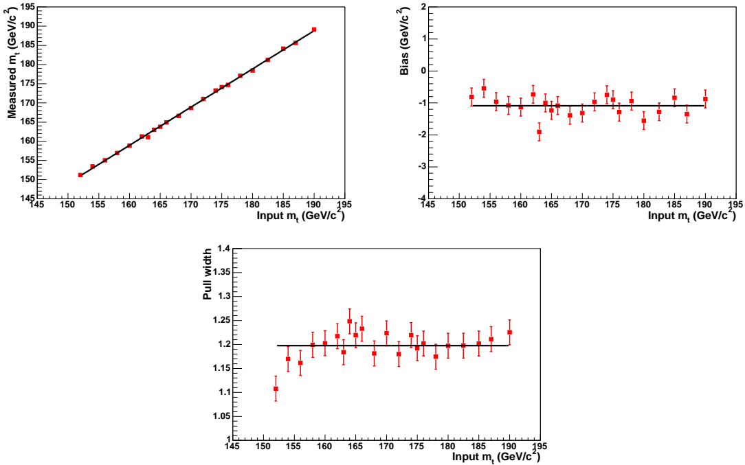
FIG. 12: Pseudoexperiment results using fully simulated signal and background events after applying a likelihood cut, with a mean of 303 events for each PE. For these samples, JES is fixed at its nominal value of 1. Top left: reconstructed vs. input top quark mass; top right: bias vs. input top quark mass; bottom: pull width vs. input top quark mass.
