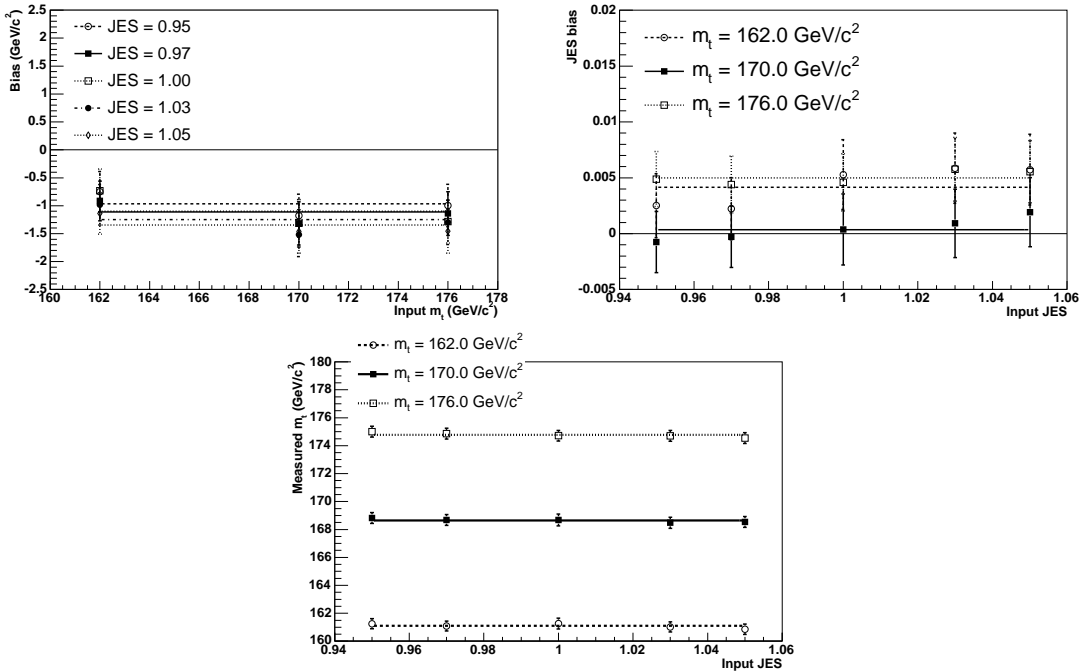
FIG. 14: Results of studying samples with shifted JES values. Top left: Mass bias vs. input top quark mass at the five different JES points; top right: JES bias vs. input JES at the three different mass points; bottom: reconstructed top quark mass vs. input JES for the three different top quark masses.
