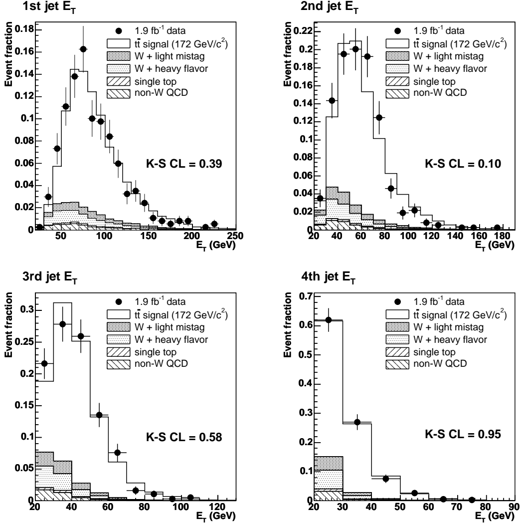
FIG. 2: Comparison of data and MC predictions for the selected events. The confidence level obtained from a K-S test on the two distributions is indicated on the histogram. The plots show, in order, the corrected E_T of the leading jet, 2nd jet, 3rd jet, and 4th jet in our events.
