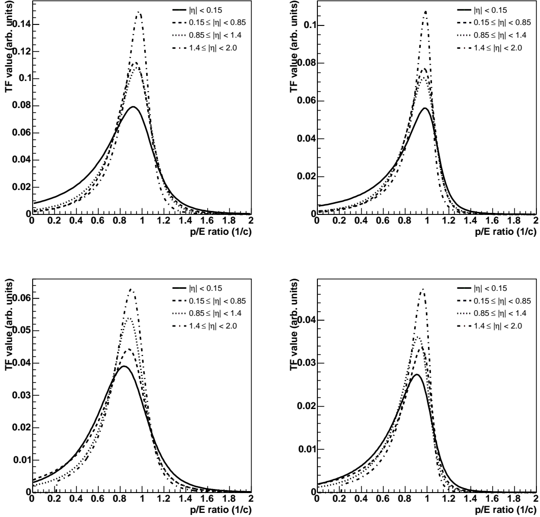
FIG. 7: Sample fitted transfer functions for light and b quarks in \eta bins. Transfer functions are shown for light quarks with parton P_T = 40 and 70 GeV/ c (top left and right, respectively), and for b quarks with parton P_T = 40 and 70 GeV/ c (bottom left and right, respectively).
