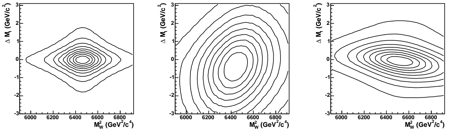
FIG. 6: Contour plots of the propagators in M_W^2 and \Delta M_t . Left: Breit-Wigner propagator, for comparison. Center: Sample effective propagator on the hadronic side of the event. Right: Sample effective propagator on the leptonic side of the event.
