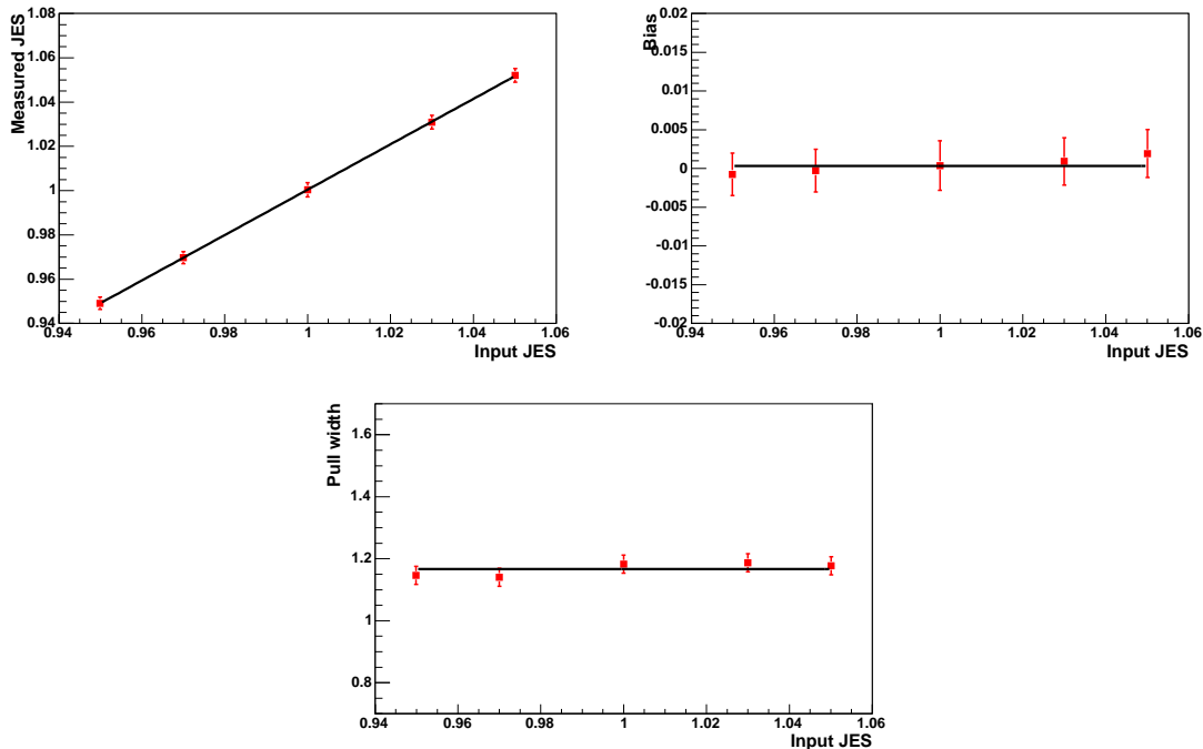
FIG. 13: JES pseudoexperiment results using fully simulated signal and background events after applying a likelihood cut, with a mean of 303 events for each PE. The top quark mass here is fixed at m_t = 170 \text{ GeV}/c^2 . Top left: reconstructed vs. input JES; top right: JES bias vs. input JES; bottom: JES pull width vs. input JES.
