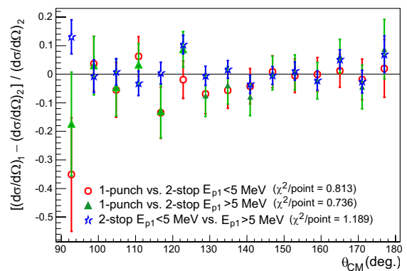
FIG. 13: The fractional differences between the absolute differential cross sections extracted for different analyzed data subsamples. The plotted error bars take into account only the independent statistical (including those from background subtractions) uncertainties for the three samples. Slightly different correction factors c_i were applied to the cross sections for different samples, as indicated in Table I, before the comparison was made.
