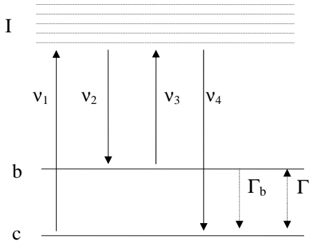
FIG. 1: CARS scheme with three input fields of frequency \nu_1 , \nu_2 and \nu_3 and a generated signal field \nu_4 = \nu_1 + \nu_3 - \nu_2 . The radiative damping rate from level b to level c is \Gamma_b and the dephasing rate of the coherence between levels b and c is \Gamma .
