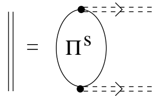
FIG. 3. Graphical representation of Eq.(45). The incoherent intensity at the position of the probe atom is the sum of all spontaneous contribution propagated through the medium.
