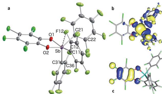
Fig. 2 Solid-state structure of stiborane 2 with thermal ellipsoids drawn at the 50% probability level (a). Select solid-state distances [Å] and angles [°]: Sb–F(12) 3.0764(16), Sb–C(11) 2.145(2), Sb–C(21) 2.126(2), Sb–C(31) 2.106(2), Sb–O(1) 2.0321(15), Sb–O(2) 1.9951(15), O(2)–Sb–C(21) 138.53(7), O(1)–Sb–C(11) 157.75(7), C(31)–Sb–F(12) 157.39(6), Sb–C(11)–C(12) 116.25(15), Sb–C(21)–C(22) 119.94(16), Sb–C(31)–C(36) 120.66(16). The HOMO (c) and LUMO (b) are the only orbitals involved in the lowest computed excitation.
