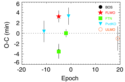
Figure 10. The residuals of the transit times from the best-fit ephemeris. The transit times are given in Table 4. The BOS observation at epoch −5 is hidden behind the FTN observation at the same epoch.
