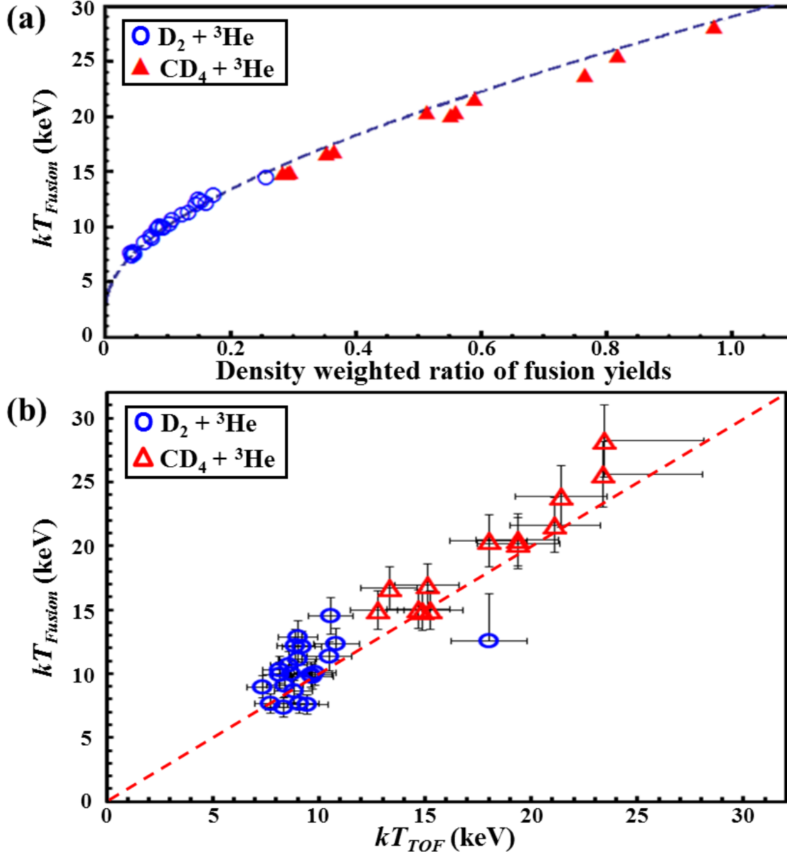
FIG. 3. (Color online) (a) Ion temperature, kT_{Fusion} , as a function of the measured density-weighted ratio of fusion yields for D_2 + {}^3He (hollow circles) and CD_4 + {}^3He (solid triangles) mixtures. The dashed line corresponds to the calculated ion temperature for a plasma size, r = 250 \mu m . (b) Comparison between kT_{Fusion} and the temperature measured by the time-of-flight method, kT_{TOF} , for D_2 + {}^3He (hollow circles) and CD_4 + {}^3He (hollow triangles) mixtures. A dashed line indicates where the temperature determined by both techniques matches.
