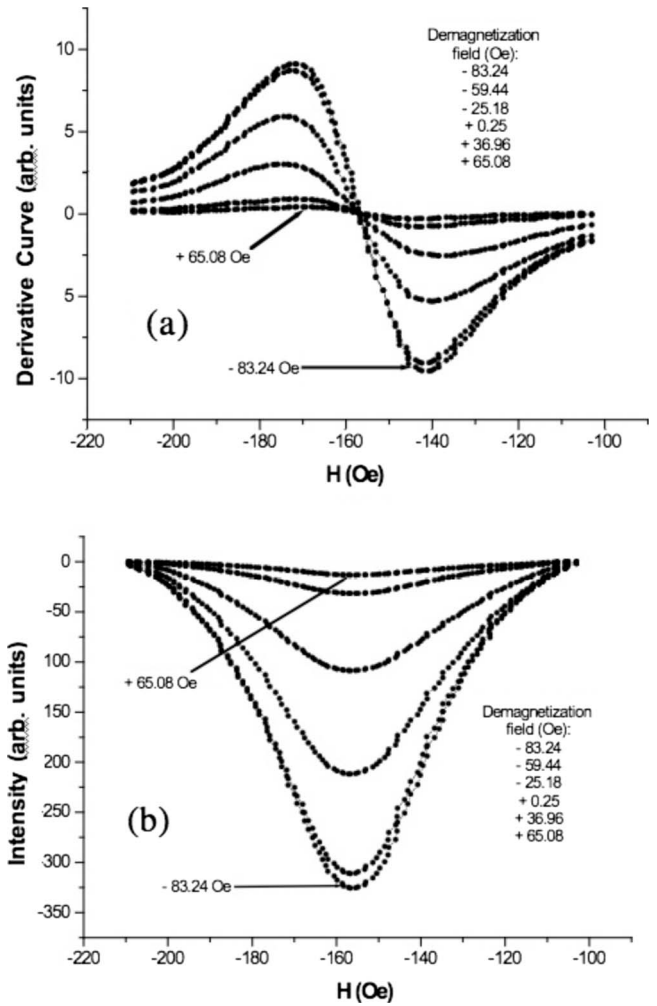
FIG. 4. The measured “disappearing behavior” of the FMR line for a frequency of 4.2 GHz. Starting with the sample saturated at a high negative field, the field is swept to a series of less negative and then positive fields (as given in the inset). The greater the excursion toward positive fields the greater the loss in signal amplitude on returning to the nominal resonant field near -155 G.
